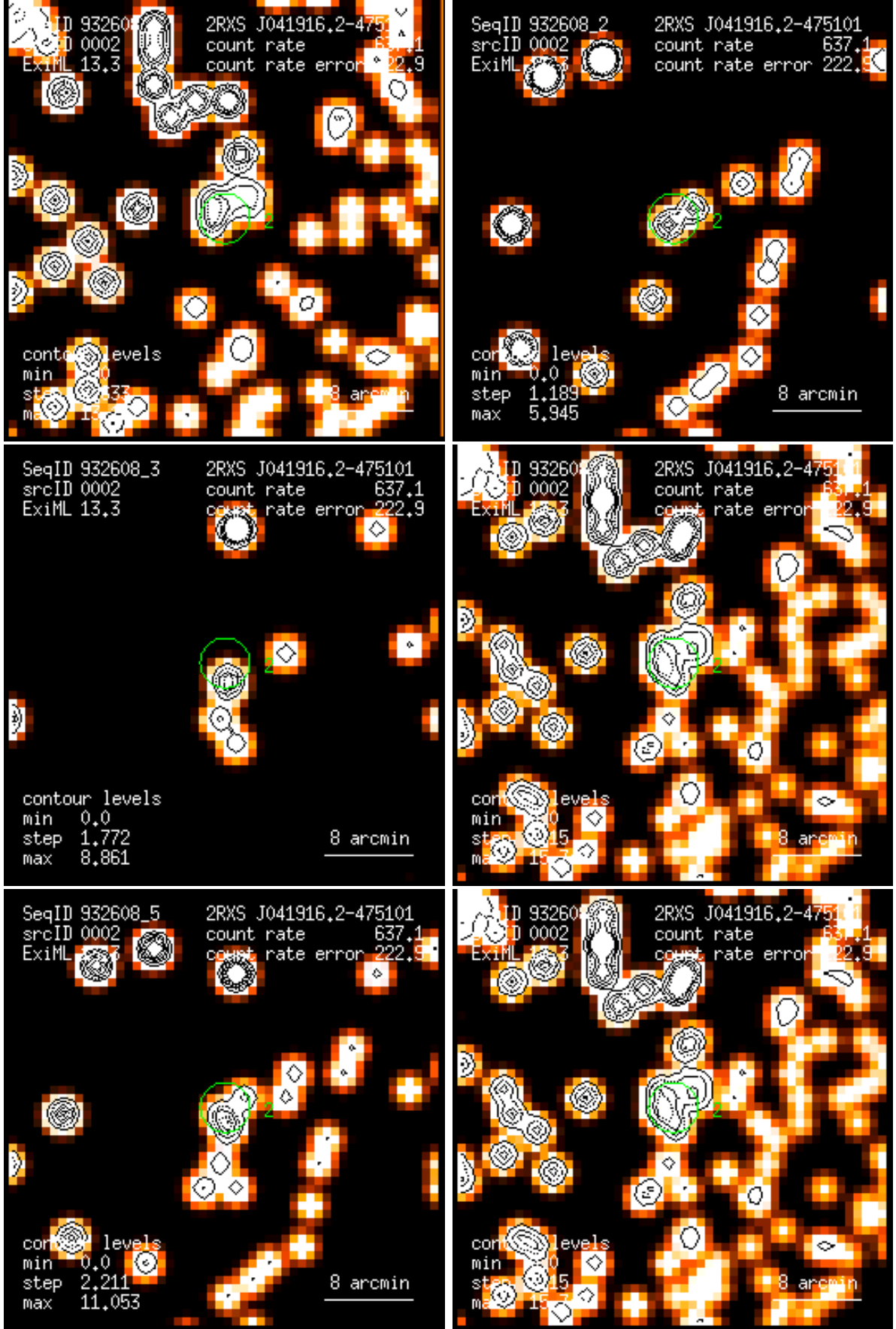
Figure 2: RASS 932608: detection 0002: band rate images, Gaussian filter: (1) PSPC channels 11 – 41, (2) 52 – 90, (3) 91 – 201, (4) 11 – 235, (5) 52 – 201, (6) 11 – 201. Broad band rates in counts/ks. Band rate contour levels in counts/ks/arcmin 2 .
