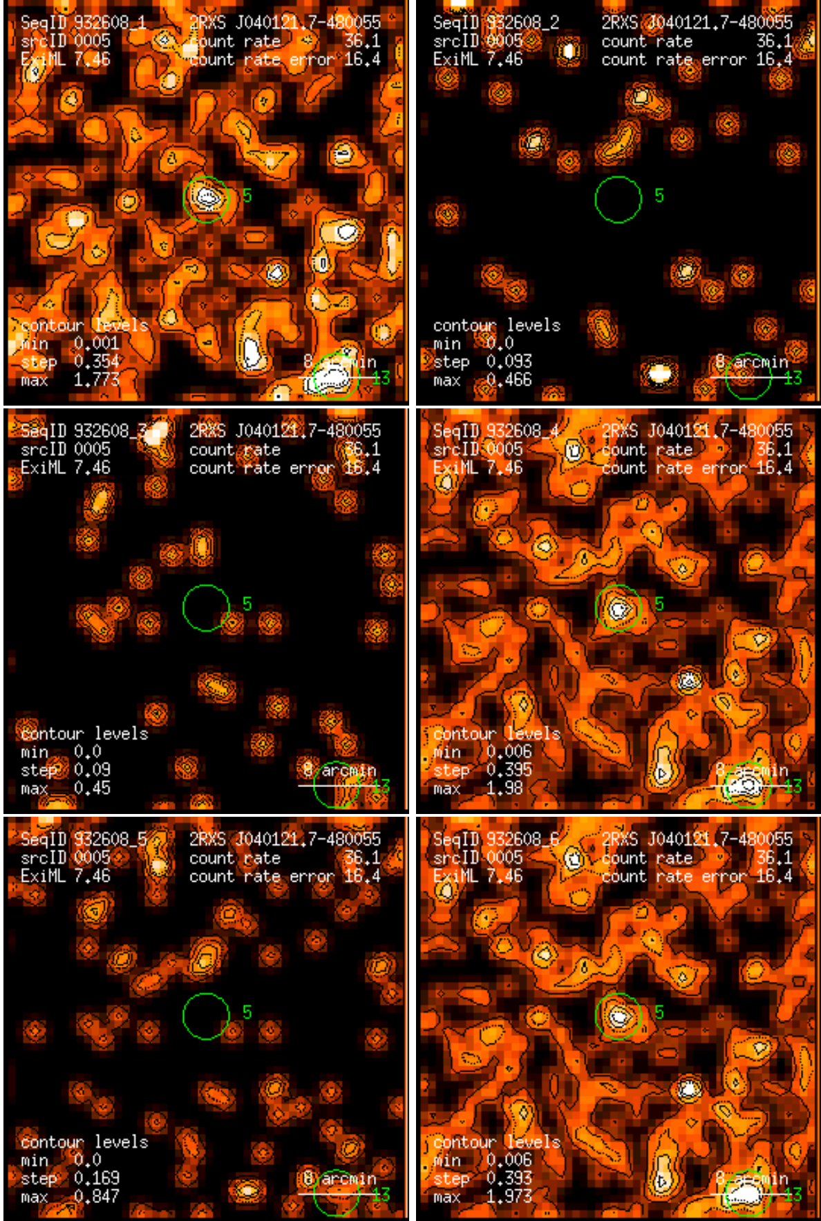
Figure 5: RASS 932608: detection 0005: band rate images, Gaussian filter: (1) PSPC channels 11 – 41, (2) 52 – 90, (3) 91 – 201, (4) 11 – 235, (5) 52 – 201, (6) 11 – 201. Broad band rates in counts/ks. Band rate contour levels in counts/ks/arcmin 2 .
