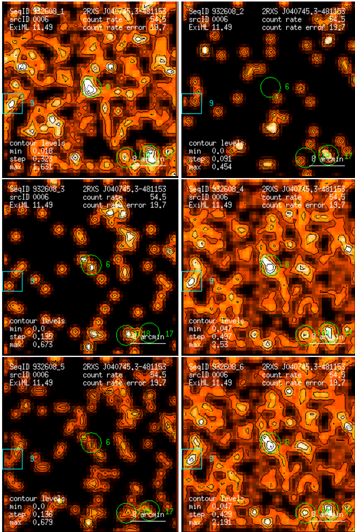
Figure 6: RASS 932608: detection 0006: band rate images, Gaussian filter: (1) PSPC channels 11 – 41, (2) 52 – 90, (3) 91 – 201, (4) 11 – 235, (5) 52 – 201, (6) 11 – 201. Broad band rates in counts/ks. Band rate contour levels in counts/ks/arcmin 2 .
