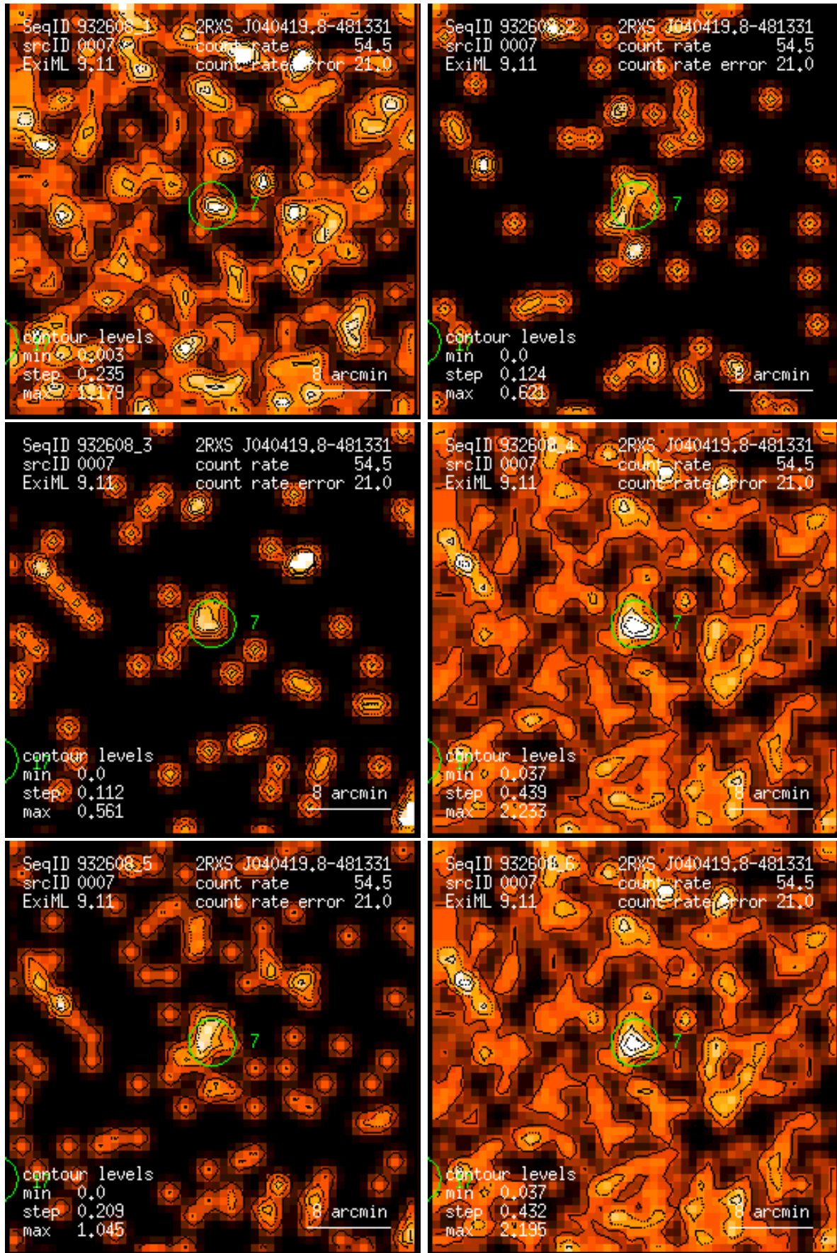
Figure 7: RASS 932608: detection 0007: band rate images, Gaussian filter: (1) PSPC channels 11 – 41, (2) 52 – 90, (3) 91 – 201, (4) 11 – 235, (5) 52 – 201, (6) 11 – 201. Broad band rates in counts/ks. Band rate contour levels in counts/ks/arcmin 2 .
