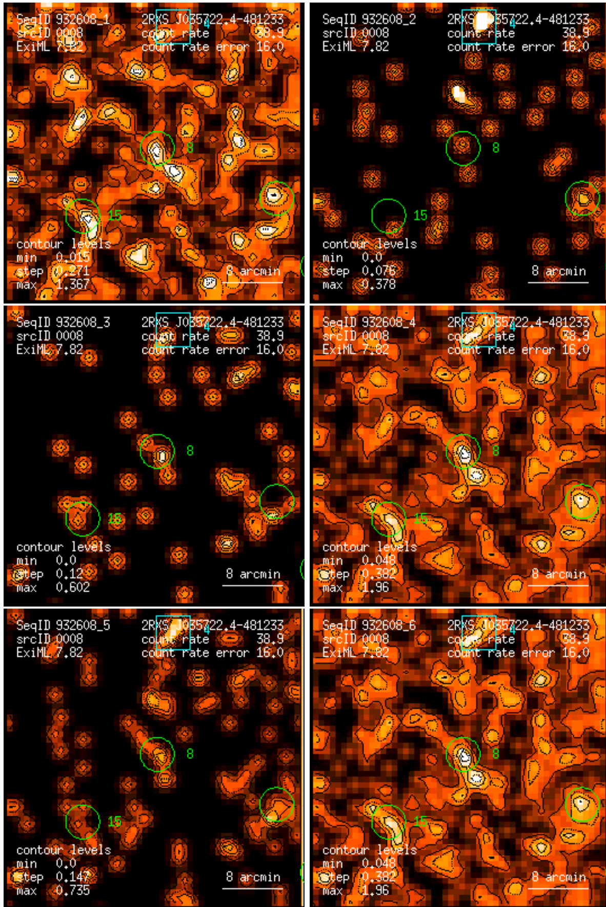
Figure 8: RASS 932608: detection 0008: band rate images, Gaussian filter: (1) PSPC channels 11 – 41, (2) 52 – 90, (3) 91 – 201, (4) 11 – 235, (5) 52 – 201, (6) 11 – 201. Broad band rates in counts/ks. Band rate contour levels in counts/ks/arcmin 2 .
