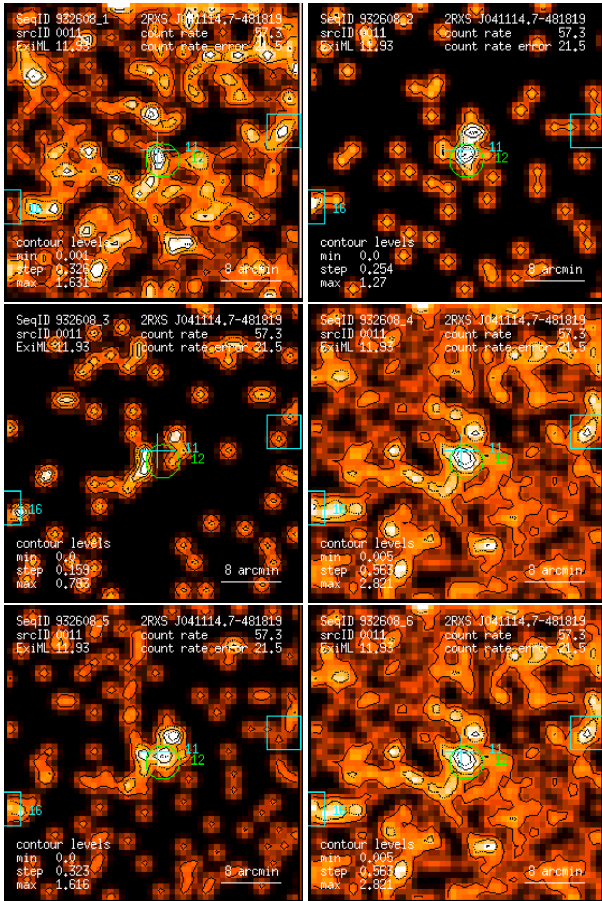
Figure 11: RASS 932608: detection 0011: band rate images, Gaussian filter: (1) PSPC channels 11 – 41, (2) 52 – 90, (3) 91 – 201, (4) 11 – 235, (5) 52 – 201, (6) 11 – 201. Broad band rates in counts/ks. Band rate contour levels in counts/ks/arcmin 2 .
