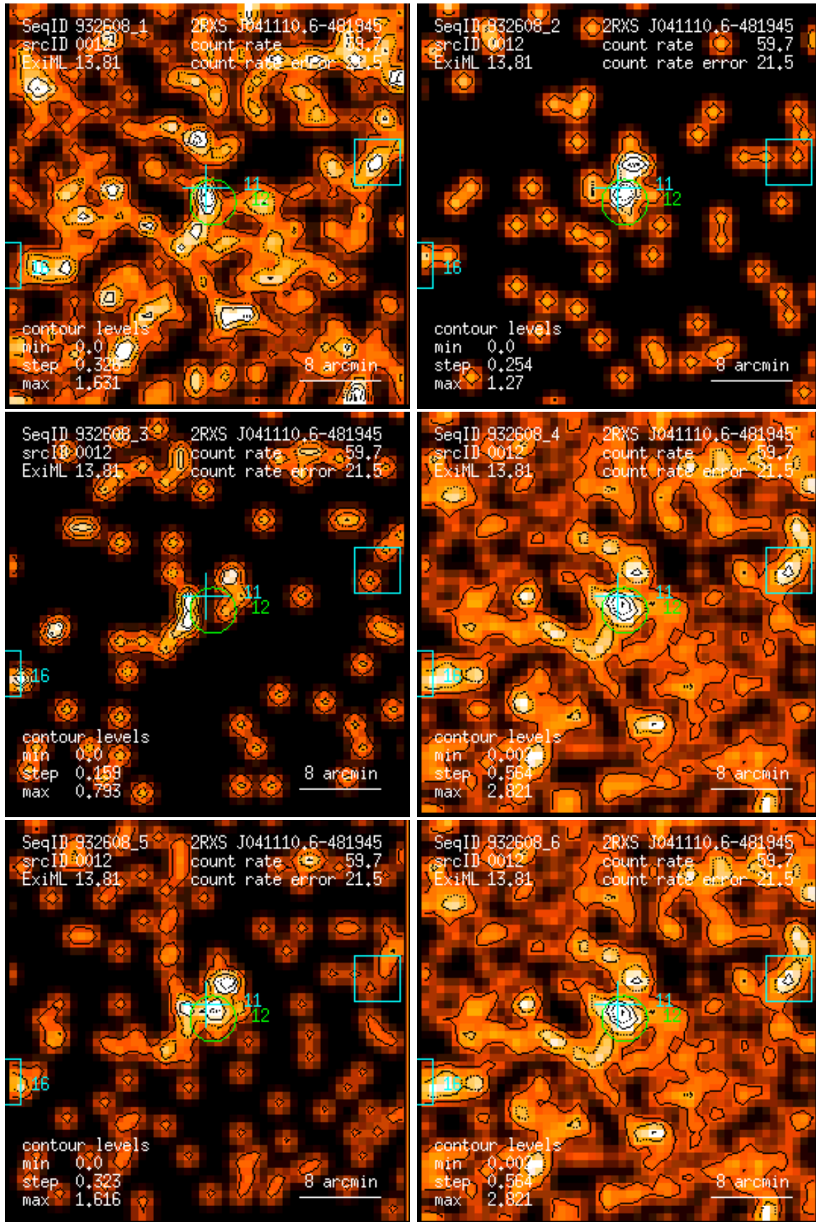
Figure 12: RASS 932608: detection 0012: band rate images, Gaussian filter: (1) PSPC channels 11 – 41, (2) 52 – 90, (3) 91 – 201, (4) 11 – 235, (5) 52 – 201, (6) 11 – 201. Broad band rates in counts/ks. Band rate contour levels in counts/ks/arcmin 2 .
