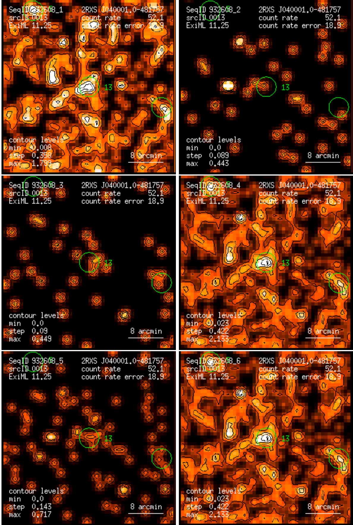
Figure 13: RASS 932608: detection 0013: band rate images, Gaussian filter: (1) PSPC channels 11 – 41, (2) 52 – 90, (3) 91 – 201, (4) 11 – 235, (5) 52 – 201, (6) 11 – 201. Broad band rates in counts/ks. Band rate contour levels in counts/ks/arcmin 2 .
