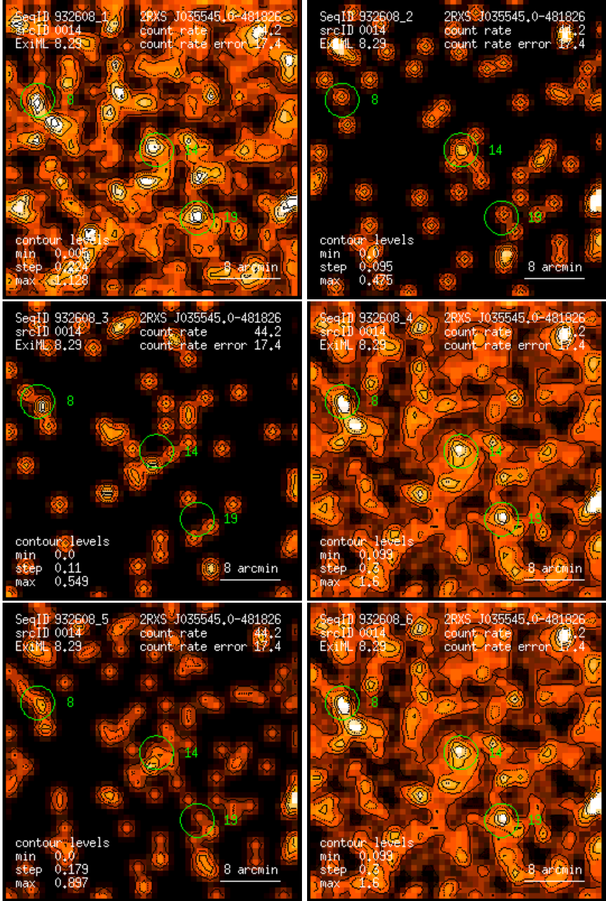
Figure 14: RASS 932608: detection 0014: band rate images, Gaussian filter: (1) PSPC channels 11 – 41, (2) 52 – 90, (3) 91 – 201, (4) 11 – 235, (5) 52 – 201, (6) 11 – 201. Broad band rates in counts/ks. Band rate contour levels in counts/ks/arcmin 2 .
