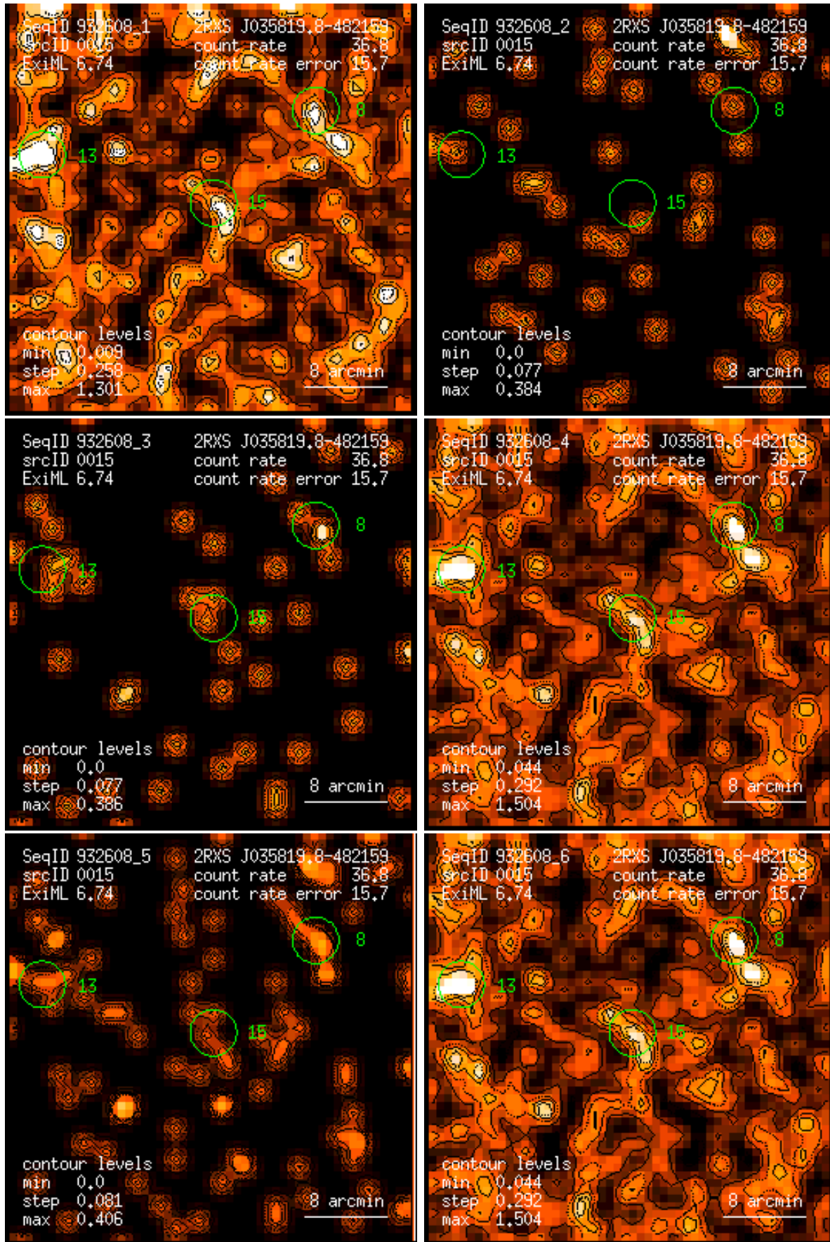
Figure 15: RASS 932608: detection 0015: band rate images, Gaussian filter: (1) PSPC channels 11 – 41, (2) 52 – 90, (3) 91 – 201, (4) 11 – 235, (5) 52 – 201, (6) 11 – 201. Broad band rates in counts/ks. Band rate contour levels in counts/ks/arcmin 2 .
