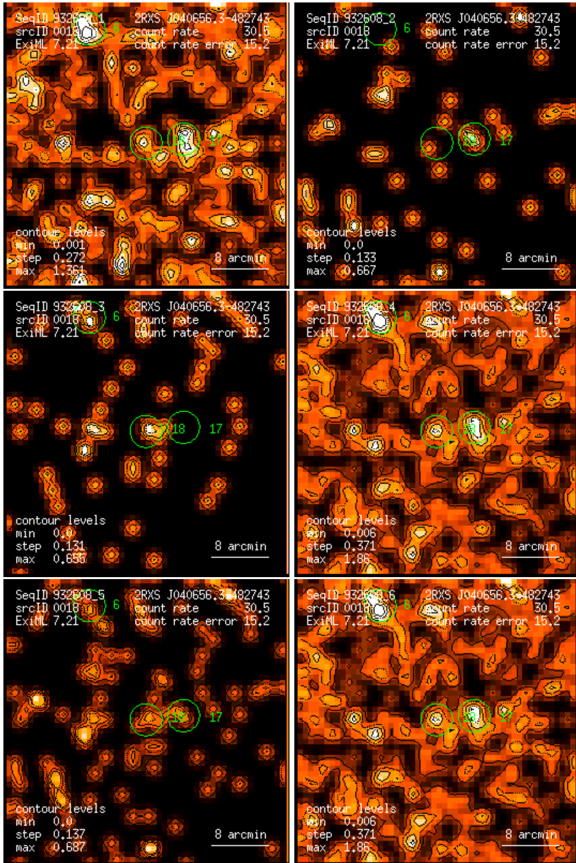
Figure 18: RASS 932608: detection 0018: band rate images, Gaussian filter: (1) PSPC channels 11 – 41, (2) 52 – 90, (3) 91 – 201, (4) 11 – 235, (5) 52 – 201, (6) 11 – 201. Broad band rates in counts/ks. Band rate contour levels in counts/ks/arcmin 2 .
