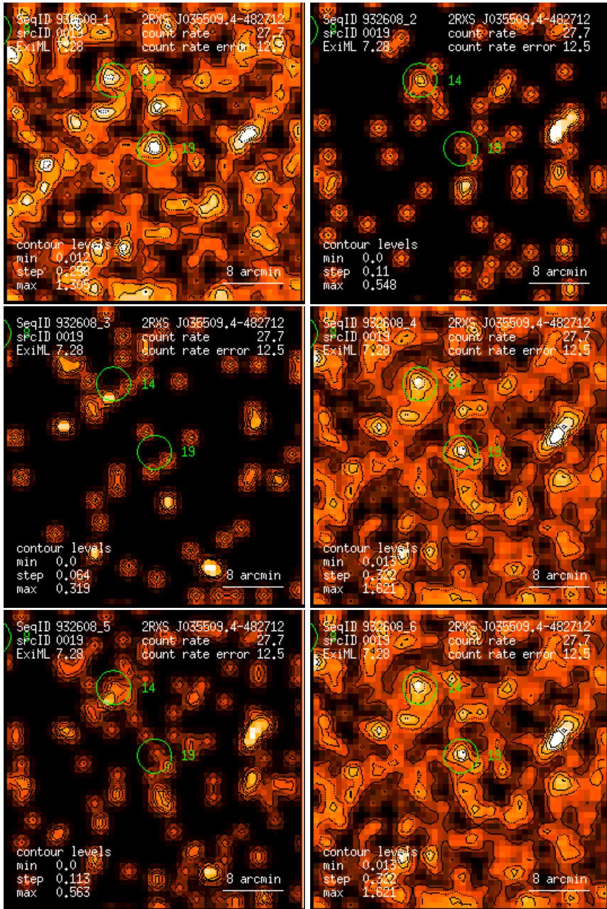
Figure 19: RASS 932608: detection 0019: band rate images, Gaussian filter: (1) PSPC channels 11 – 41, (2) 52 – 90, (3) 91 – 201, (4) 11 – 235, (5) 52 – 201, (6) 11 – 201. Broad band rates in counts/ks. Band rate contour levels in counts/ks/arcmin 2 .
