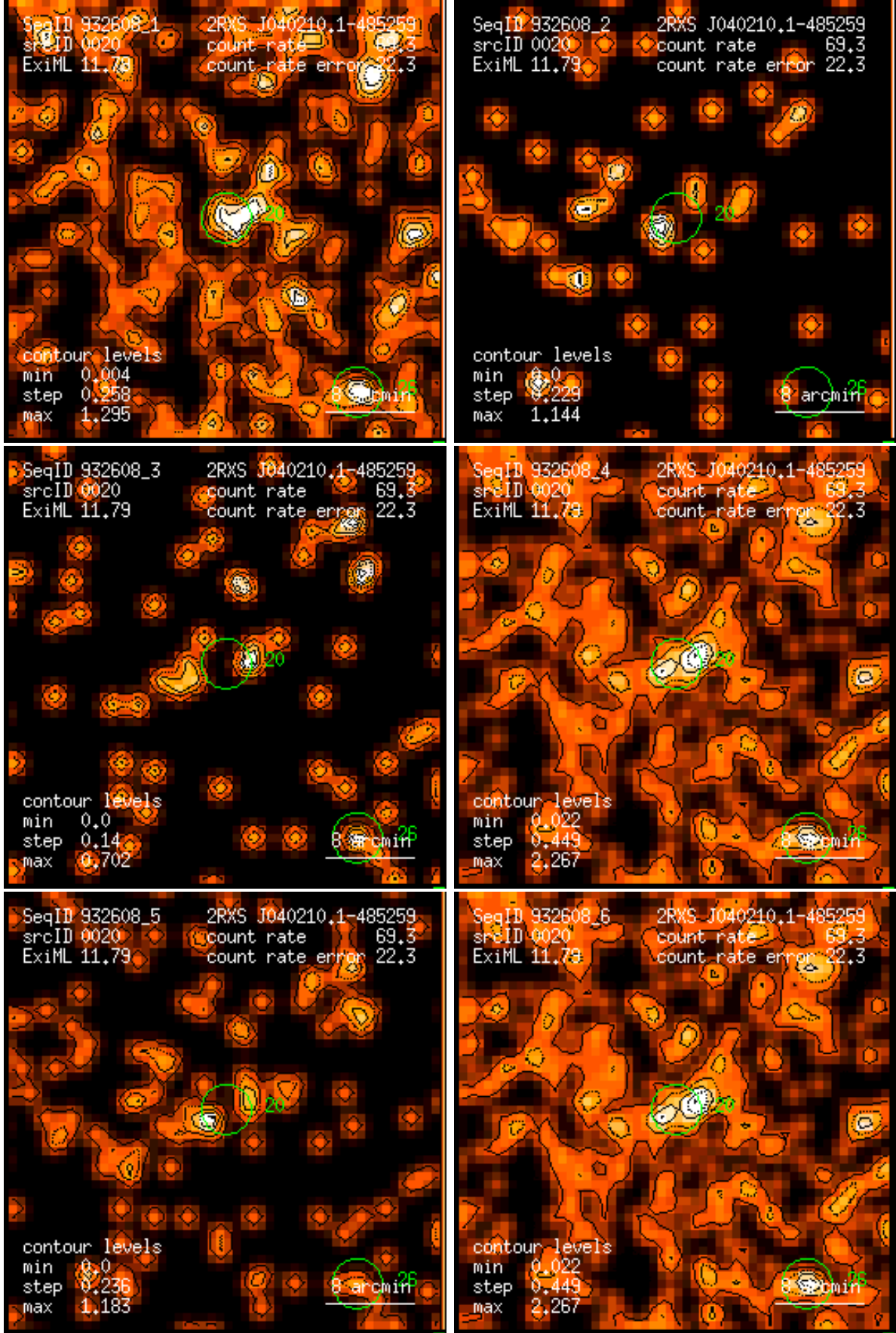
Figure 20: RASS 932608: detection 0020: band rate images, Gaussian filter: (1) PSPC channels 11 – 41, (2) 52 – 90, (3) 91 – 201, (4) 11 – 235, (5) 52 – 201, (6) 11 – 201. Broad band rates in counts/ks. Band rate contour levels in counts/ks/arcmin 2 .
