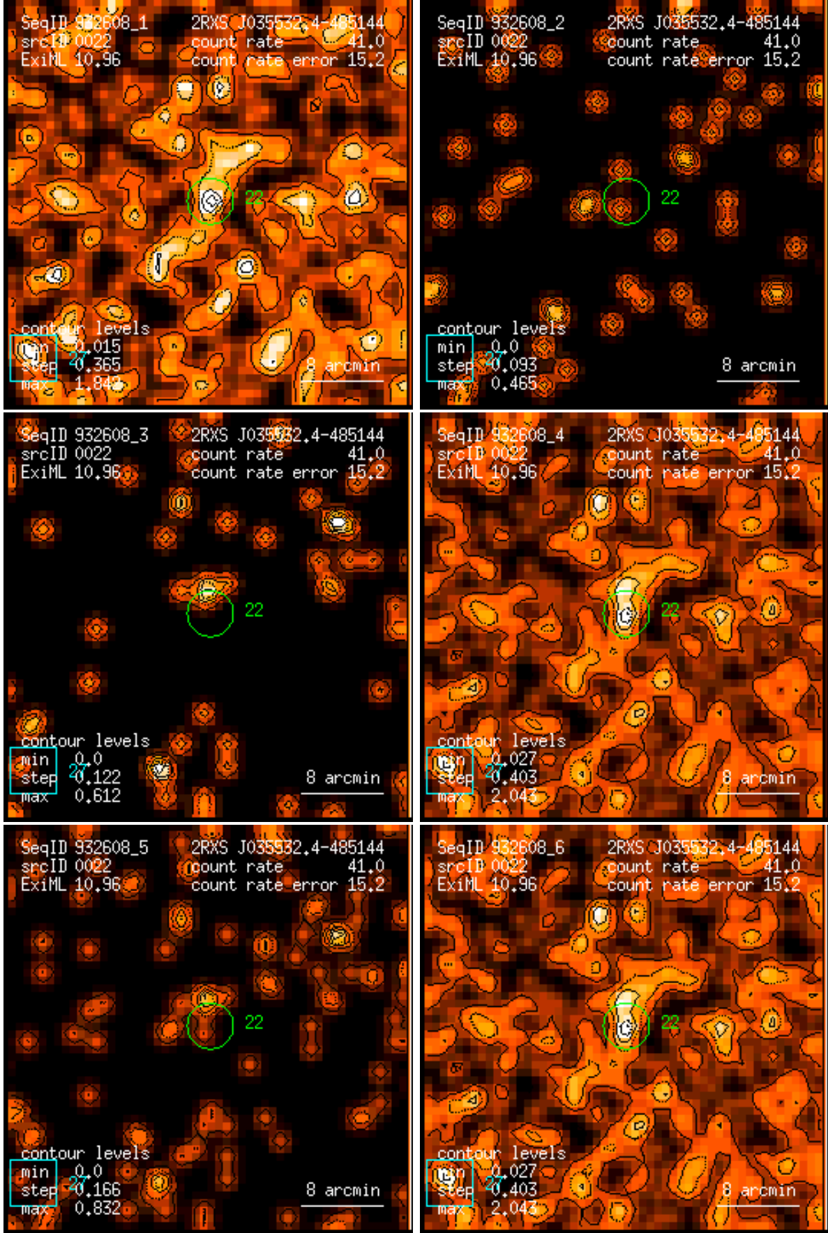
Figure 22: RASS 932608: detection 0022: band rate images, Gaussian filter: (1) PSPC channels 11 – 41, (2) 52 – 90, (3) 91 – 201, (4) 11 – 235, (5) 52 – 201, (6) 11 – 201. Broad band rates in counts/ks. Band rate contour levels in counts/ks/arcmin 2 .
