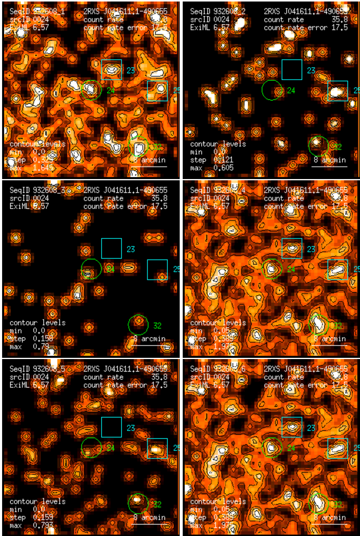
Figure 24: RASS 932608: detection 0024: band rate images, Gaussian filter: (1) PSPC channels 11 – 41, (2) 52 – 90, (3) 91 – 201, (4) 11 – 235, (5) 52 – 201, (6) 11 – 201. Broad band rates in counts/ks. Band rate contour levels in counts/ks/arcmin 2 .
