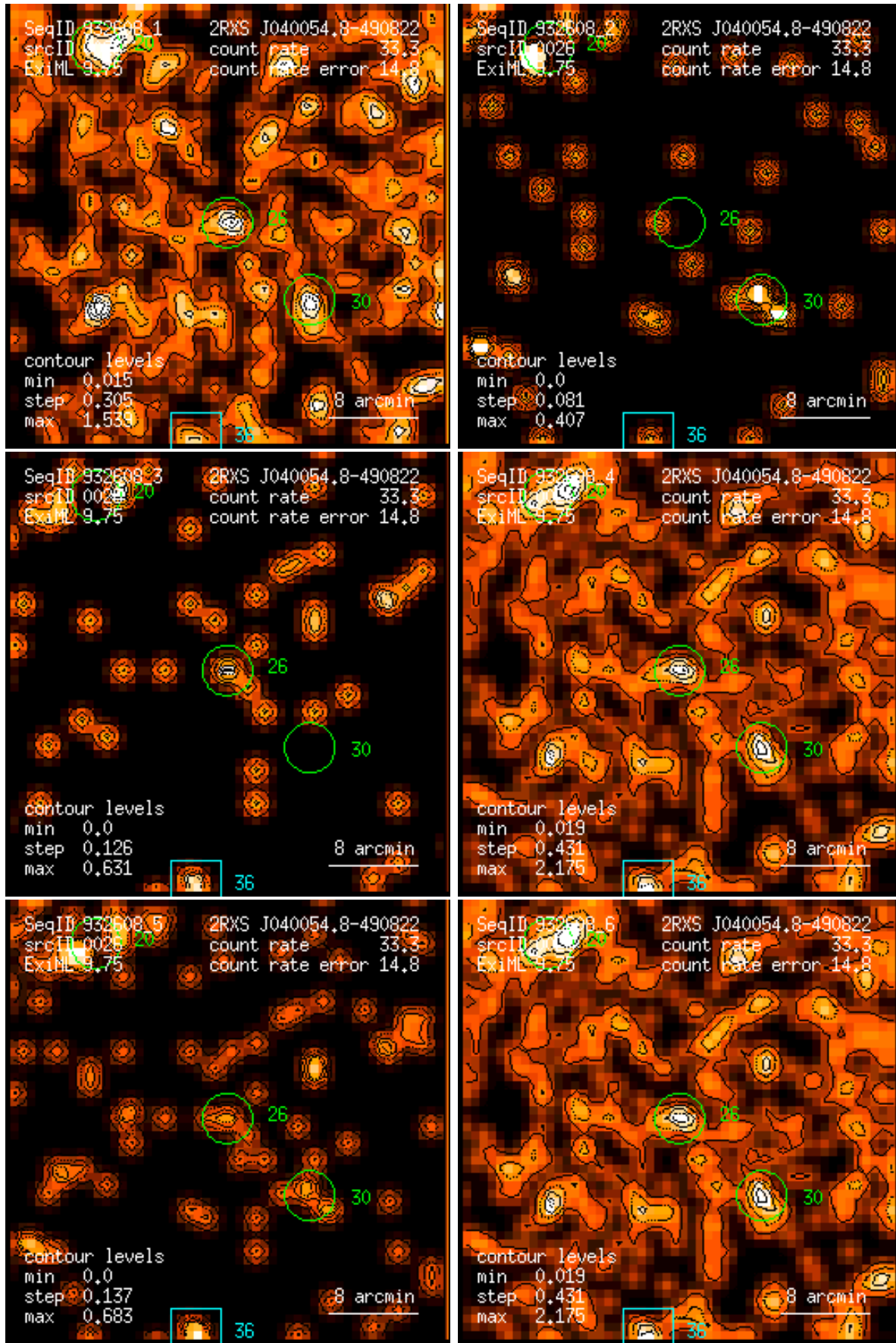
Figure 26: RASS 932608: detection 0026: band rate images, Gaussian filter: (1) PSPC channels 11 – 41, (2) 52 – 90, (3) 91 – 201, (4) 11 – 235, (5) 52 – 201, (6) 11 – 201. Broad band rates in counts/ks. Band rate contour levels in counts/ks/arcmin 2 .
