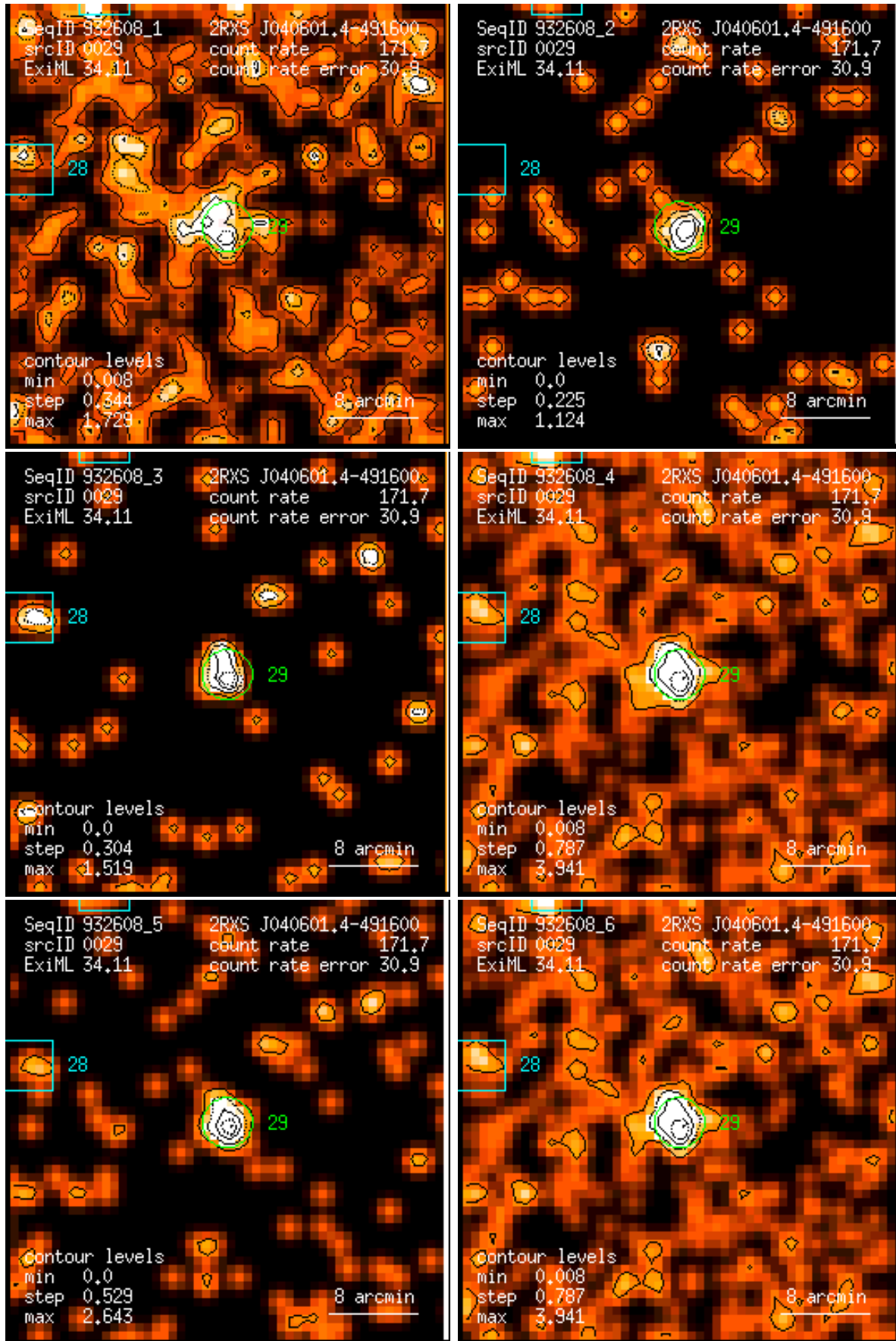
Figure 29: RASS 932608: detection 0029: band rate images, Gaussian filter: (1) PSPC channels 11 – 41, (2) 52 – 90, (3) 91 – 201, (4) 11 – 235, (5) 52 – 201, (6) 11 – 201. Broad band rates in counts/ks. Band rate contour levels in counts/ks/arcmin 2 .
