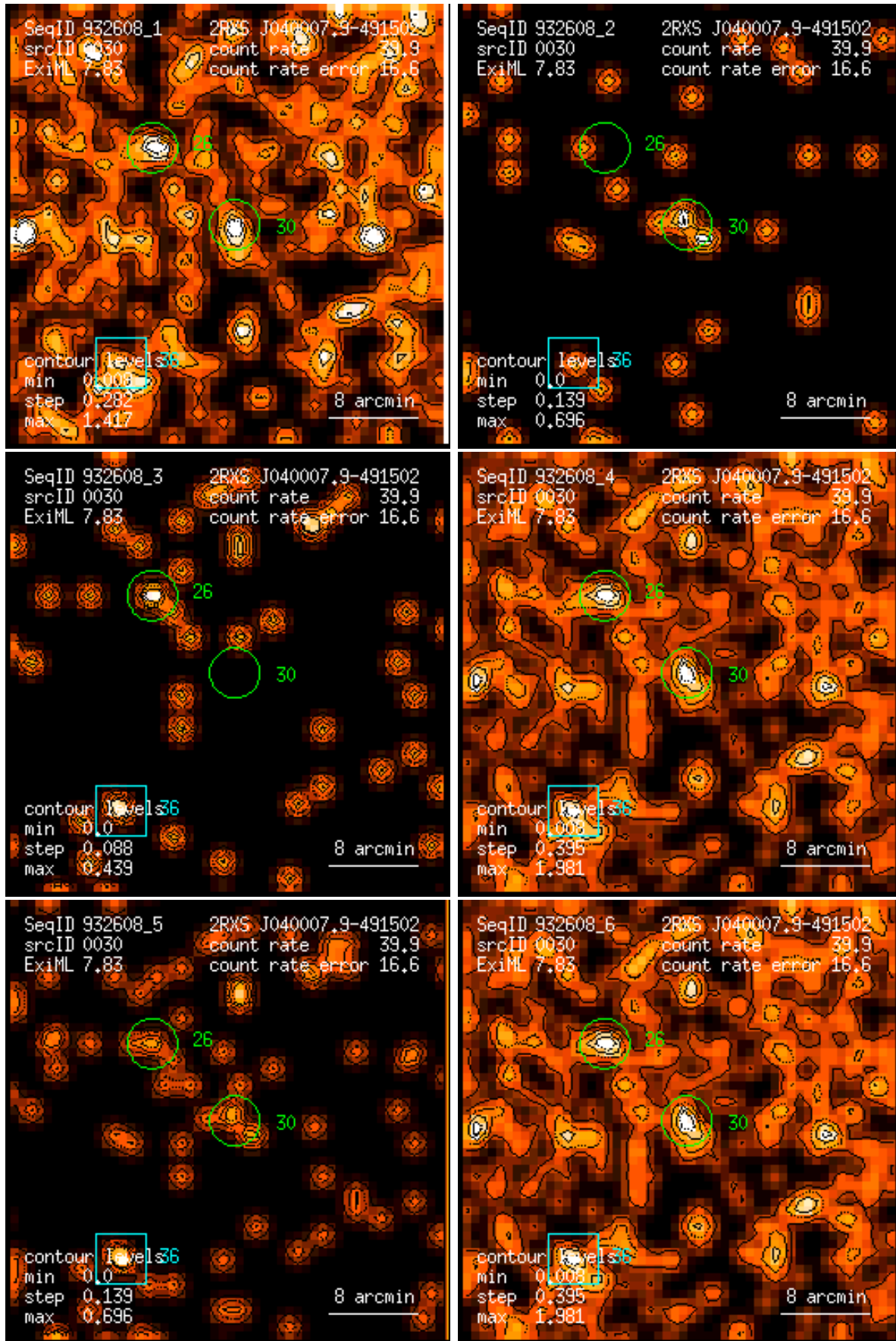
Figure 30: RASS 932608: detection 0030: band rate images, Gaussian filter: (1) PSPC channels 11 – 41, (2) 52 – 90, (3) 91 – 201, (4) 11 – 235, (5) 52 – 201, (6) 11 – 201. Broad band rates in counts/ks. Band rate contour levels in counts/ks/arcmin 2 .
