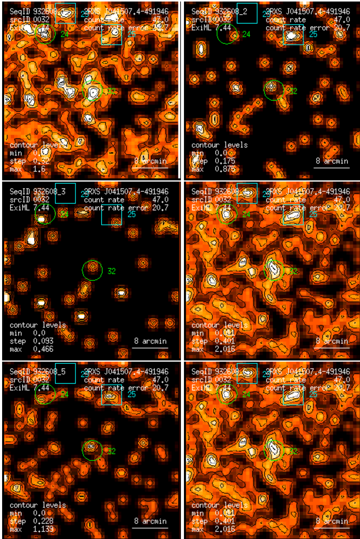
Figure 32: RASS 932608: detection 0032: band rate images, Gaussian filter: (1) PSPC channels 11 – 41, (2) 52 – 90, (3) 91 – 201, (4) 11 – 235, (5) 52 – 201, (6) 11 – 201. Broad band rates in counts/ks. Band rate contour levels in counts/ks/arcmin 2 .
