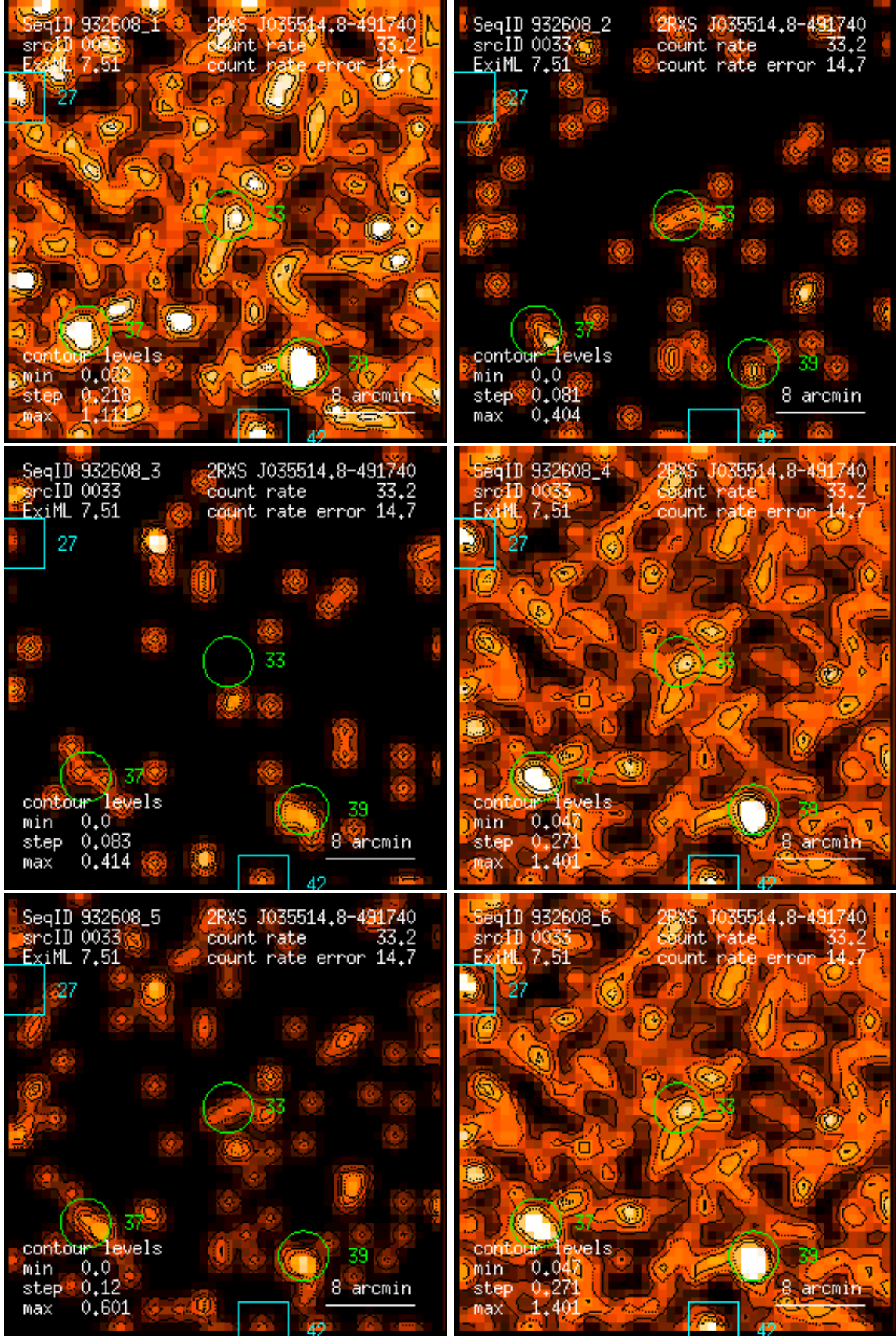
Figure 33: RASS 932608: detection 0033: band rate images, Gaussian filter: (1) PSPC channels 11 – 41, (2) 52 – 90, (3) 91 – 201, (4) 11 – 235, (5) 52 – 201, (6) 11 – 201. Broad band rates in counts/ks. Band rate contour levels in counts/ks/arcmin 2 .
