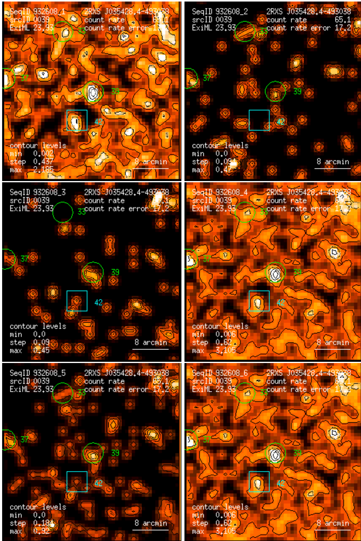
Figure 39: RASS 932608: detection 0039: band rate images, Gaussian filter: (1) PSPC channels 11 – 41, (2) 52 – 90, (3) 91 – 201, (4) 11 – 235, (5) 52 – 201, (6) 11 – 201. Broad band rates in counts/ks. Band rate contour levels in counts/ks/arcmin 2 .
