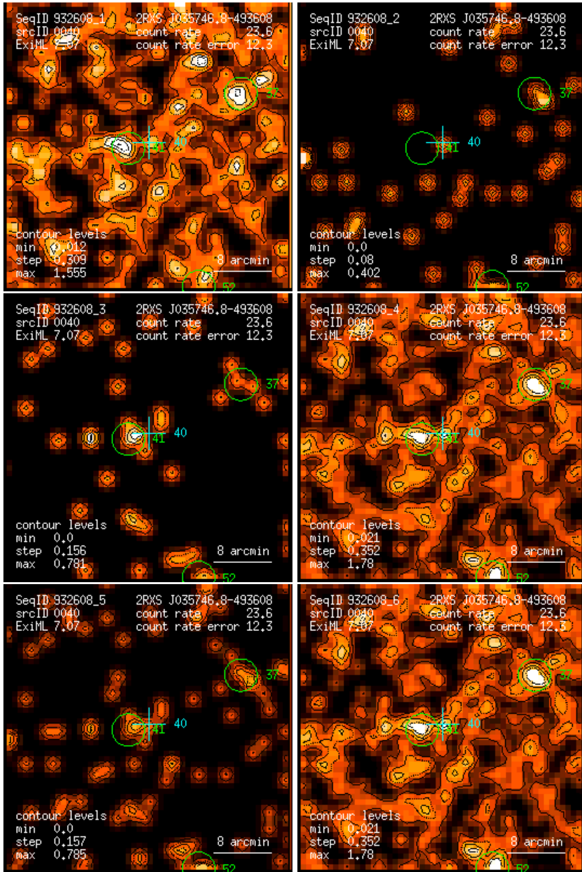
Figure 40: RASS 932608: detection 0040: band rate images, Gaussian filter: (1) PSPC channels 11 – 41, (2) 52 – 90, (3) 91 – 201, (4) 11 – 235, (5) 52 – 201, (6) 11 – 201. Broad band rates in counts/ks. Band rate contour levels in counts/ks/arcmin 2 .
