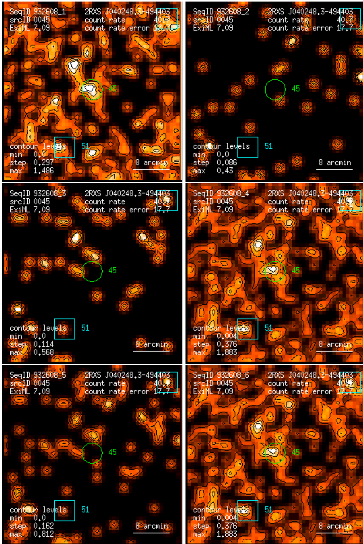
Figure 45: RASS 932608: detection 0045: band rate images, Gaussian filter: (1) PSPC channels 11 – 41, (2) 52 – 90, (3) 91 – 201, (4) 11 – 235, (5) 52 – 201, (6) 11 – 201. Broad band rates in counts/ks. Band rate contour levels in counts/ks/arcmin 2 .
