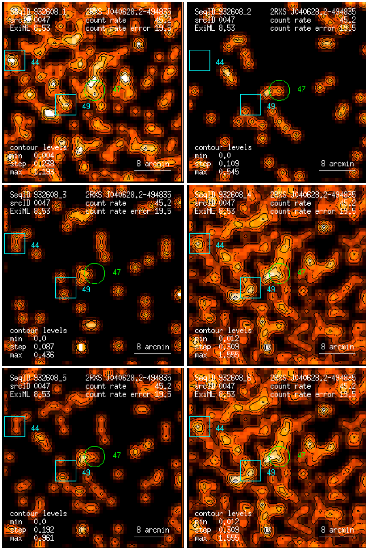
Figure 47: RASS 932608: detection 0047: band rate images, Gaussian filter: (1) PSPC channels 11 – 41, (2) 52 – 90, (3) 91 – 201, (4) 11 – 235, (5) 52 – 201, (6) 11 – 201. Broad band rates in counts/ks. Band rate contour levels in counts/ks/arcmin 2 .
