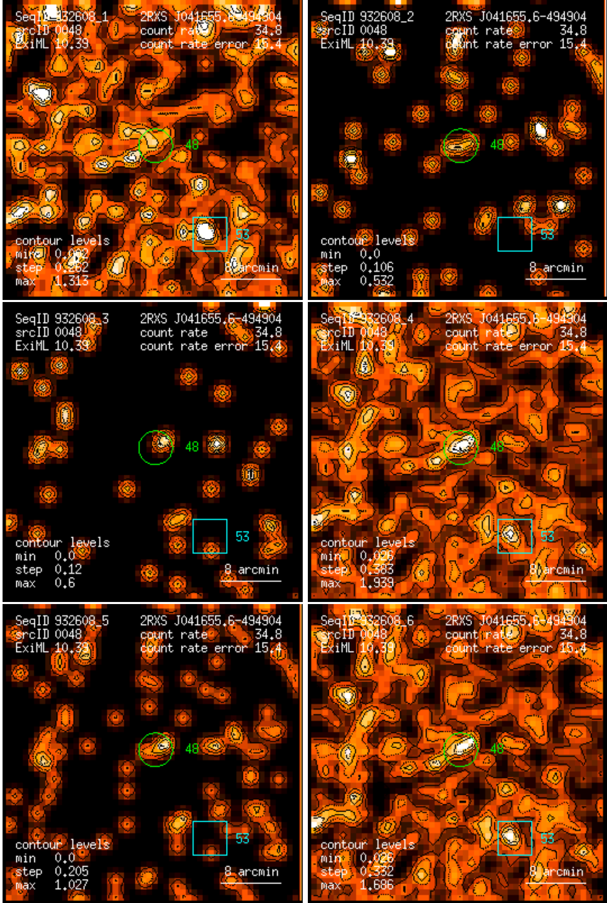
Figure 48: RASS 932608: detection 0048: band rate images, Gaussian filter: (1) PSPC channels 11 – 41, (2) 52 – 90, (3) 91 – 201, (4) 11 – 235, (5) 52 – 201, (6) 11 – 201. Broad band rates in counts/ks. Band rate contour levels in counts/ks/arcmin 2 .
