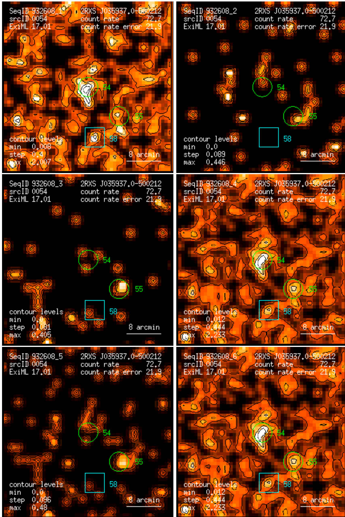
Figure 54: RASS 932608: detection 0054: band rate images, Gaussian filter: (1) PSPC channels 11 – 41, (2) 52 – 90, (3) 91 – 201, (4) 11 – 235, (5) 52 – 201, (6) 11 – 201. Broad band rates in counts/ks. Band rate contour levels in counts/ks/arcmin 2 .
