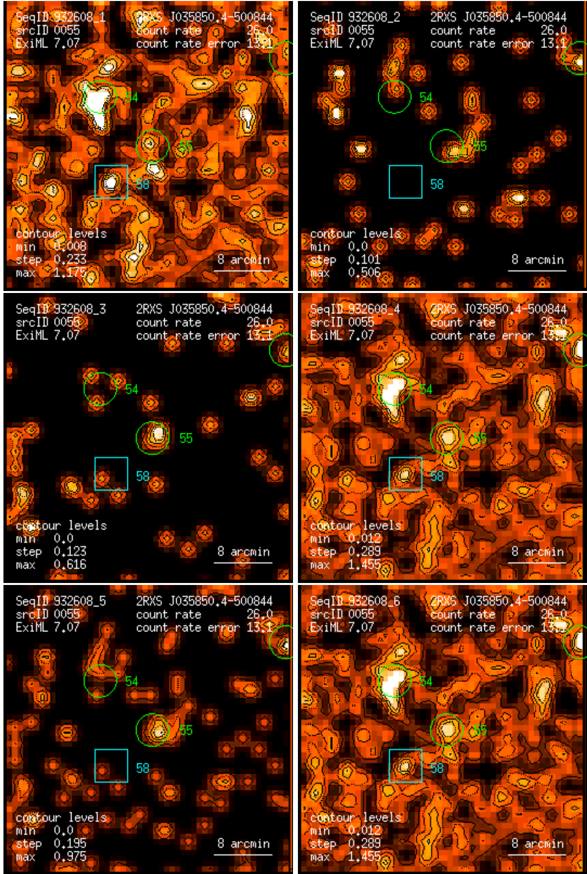
Figure 55: RASS 932608: detection 0055: band rate images, Gaussian filter: (1) PSPC channels 11 – 41, (2) 52 – 90, (3) 91 – 201, (4) 11 – 235, (5) 52 – 201, (6) 11 – 201. Broad band rates in counts/ks. Band rate contour levels in counts/ks/arcmin 2 .
