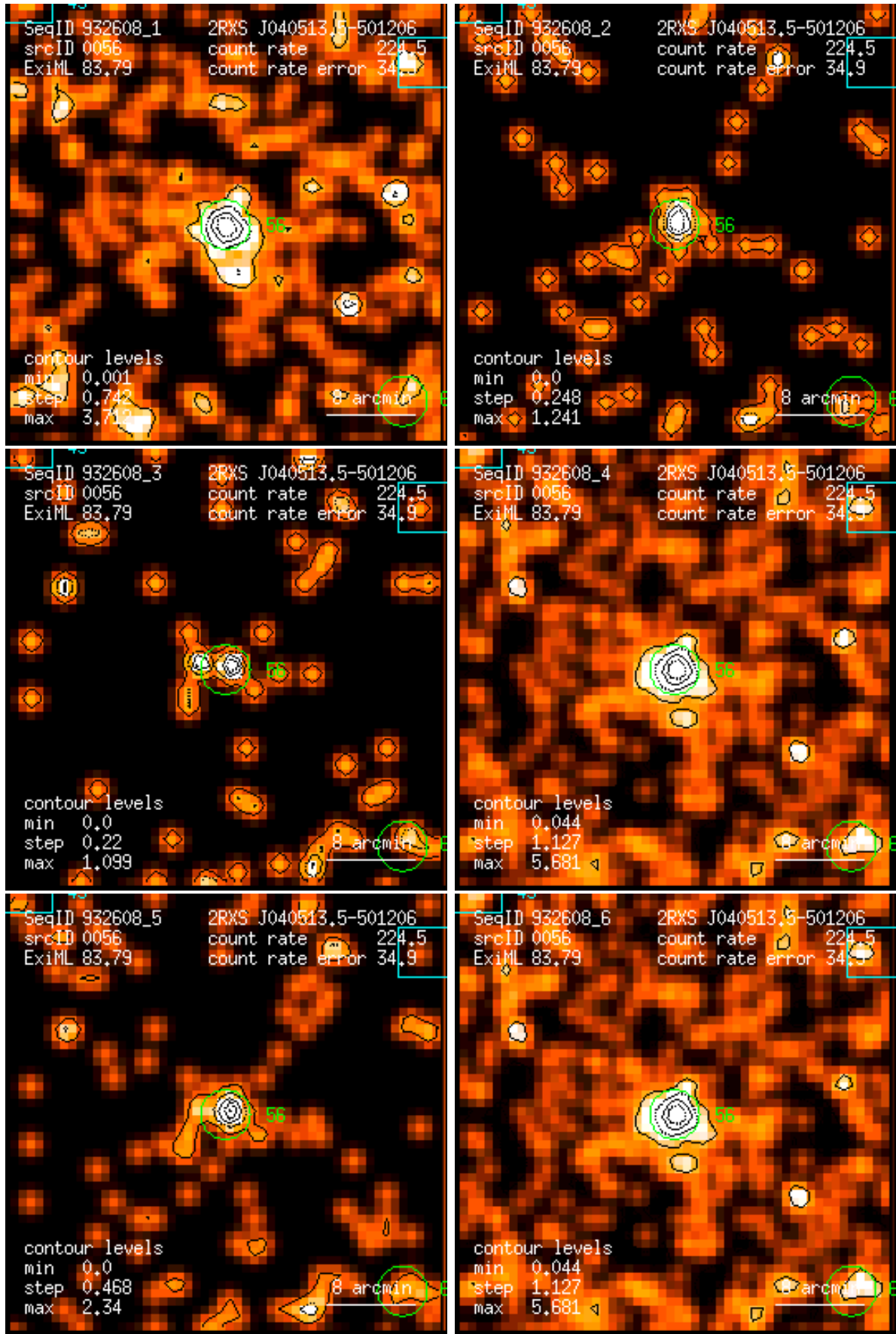
Figure 56: RASS 932608: detection 0056: band rate images, Gaussian filter: (1) PSPC channels 11 – 41, (2) 52 – 90, (3) 91 – 201, (4) 11 – 235, (5) 52 – 201, (6) 11 – 201. Broad band rates in counts/ks. Band rate contour levels in counts/ks/arcmin 2 .
