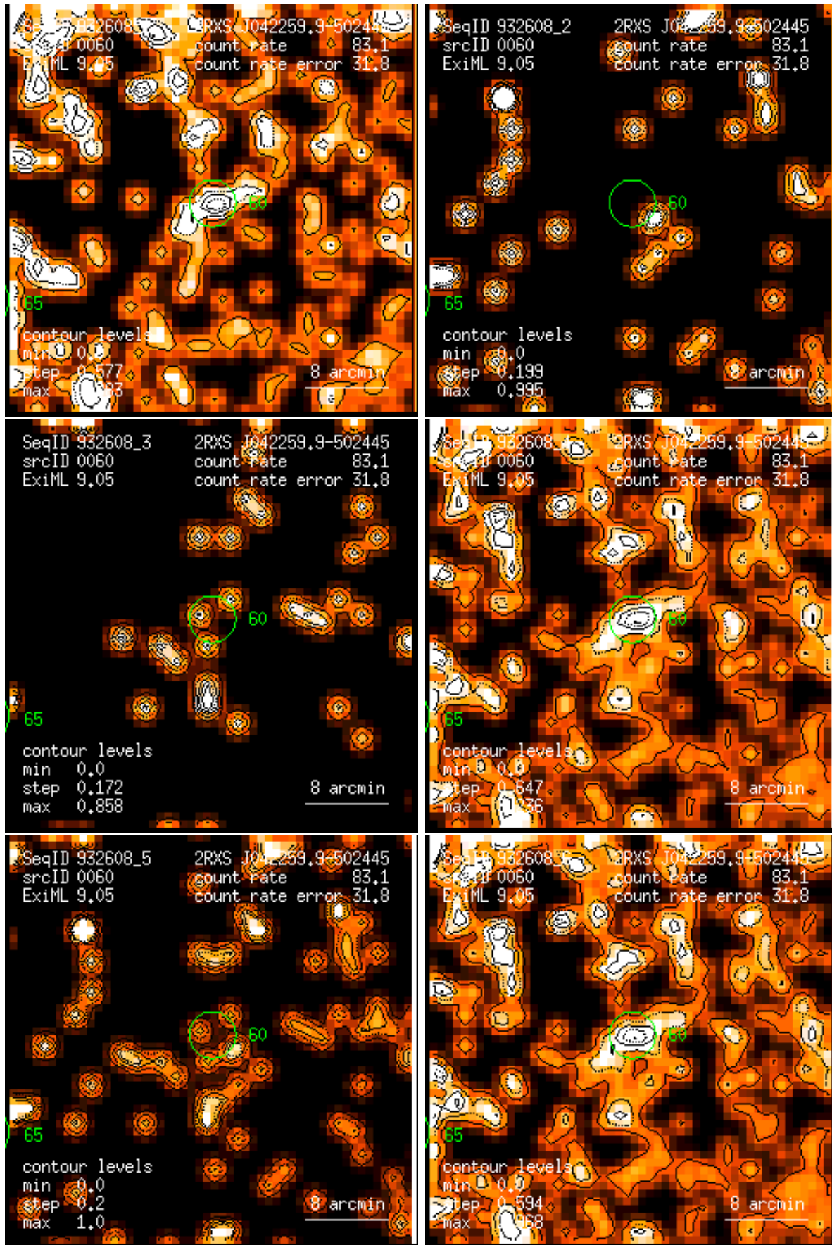
Figure 60: RASS 932608: detection 0060: band rate images, Gaussian filter: (1) PSPC channels 11 – 41, (2) 52 – 90, (3) 91 – 201, (4) 11 – 235, (5) 52 – 201, (6) 11 – 201. Broad band rates in counts/ks. Band rate contour levels in counts/ks/arcmin 2 .
