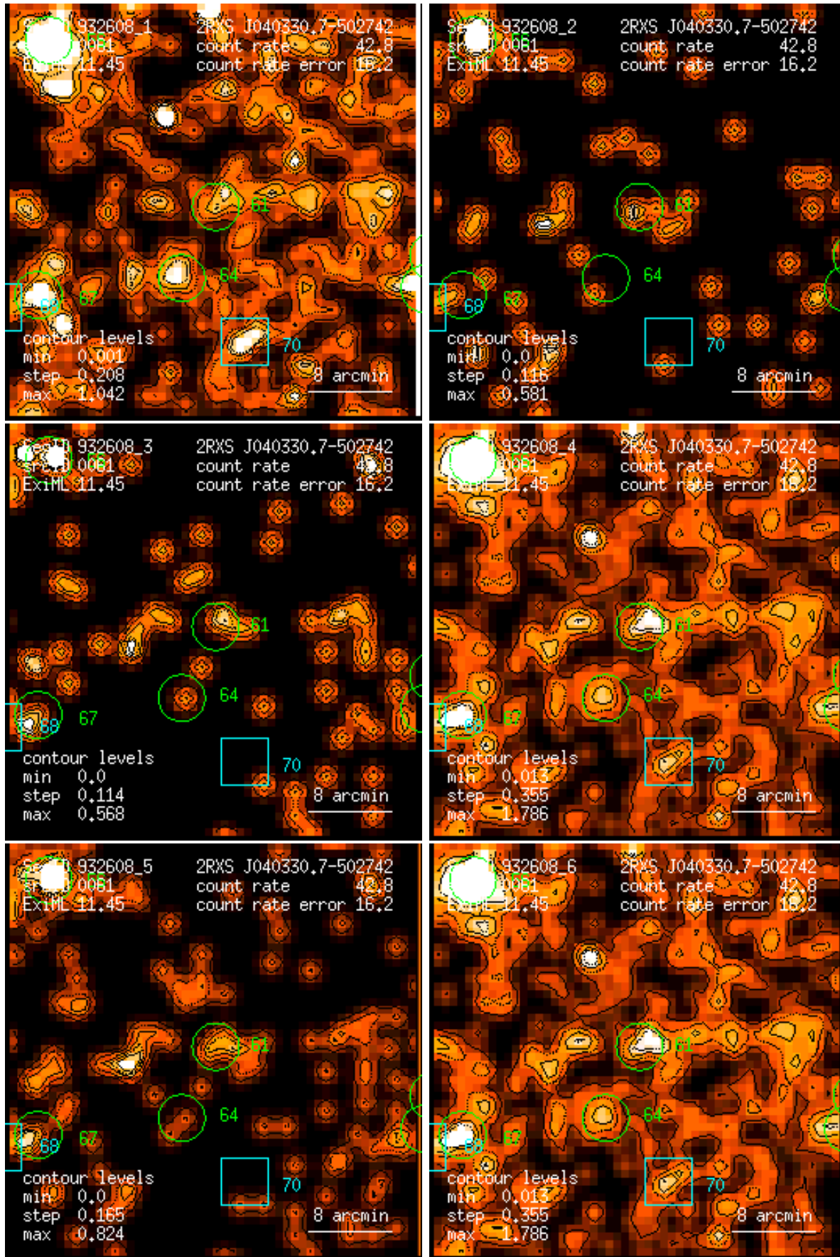
Figure 61: RASS 932608: detection 0061: band rate images, Gaussian filter: (1) PSPC channels 11 – 41, (2) 52 – 90, (3) 91 – 201, (4) 11 – 235, (5) 52 – 201, (6) 11 – 201. Broad band rates in counts/ks. Band rate contour levels in counts/ks/arcmin 2 .
