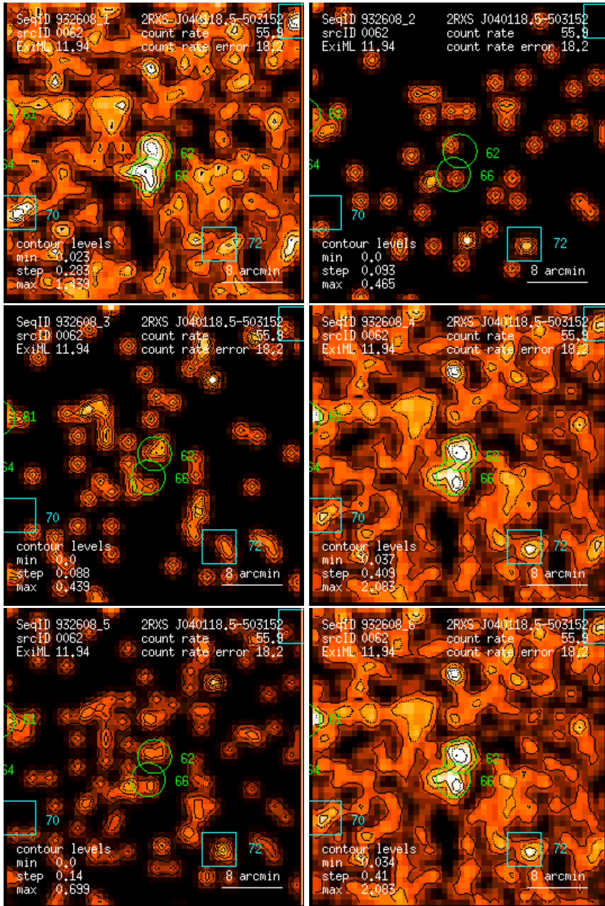
Figure 62: RASS 932608: detection 0062: band rate images, Gaussian filter: (1) PSPC channels 11 – 41, (2) 52 – 90, (3) 91 – 201, (4) 11 – 235, (5) 52 – 201, (6) 11 – 201. Broad band rates in counts/ks. Band rate contour levels in counts/ks/arcmin 2 .
