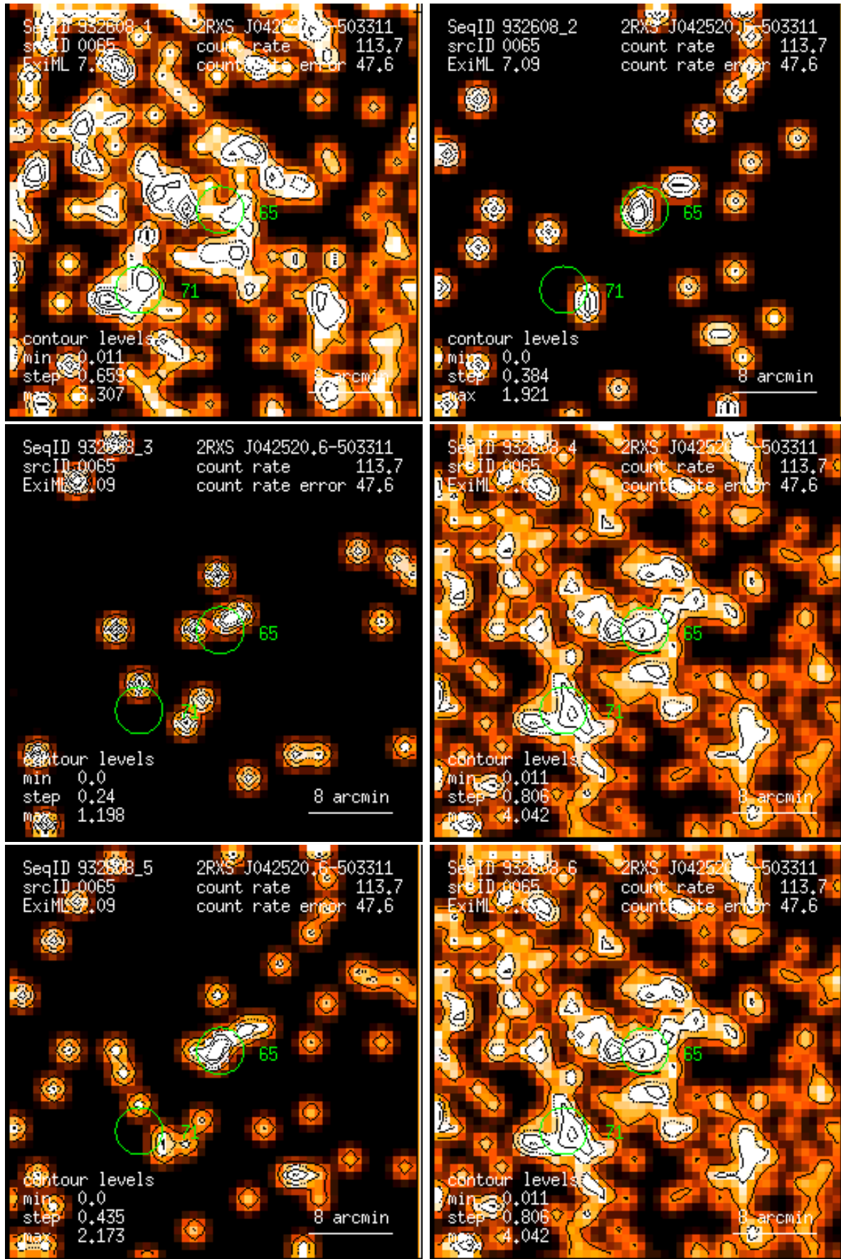
Figure 65: RASS 932608: detection 0065: band rate images, Gaussian filter: (1) PSPC channels 11 – 41, (2) 52 – 90, (3) 91 – 201, (4) 11 – 235, (5) 52 – 201, (6) 11 – 201. Broad band rates in counts/ks. Band rate contour levels in counts/ks/arcmin 2 .
