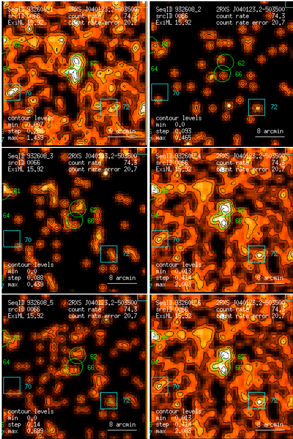
Figure 66: RASS 932608: detection 0066: band rate images, Gaussian filter: (1) PSPC channels 11 – 41, (2) 52 – 90, (3) 91 – 201, (4) 11 – 235, (5) 52 – 201, (6) 11 – 201. Broad band rates in counts/ks. Band rate contour levels in counts/ks/arcmin 2 .
