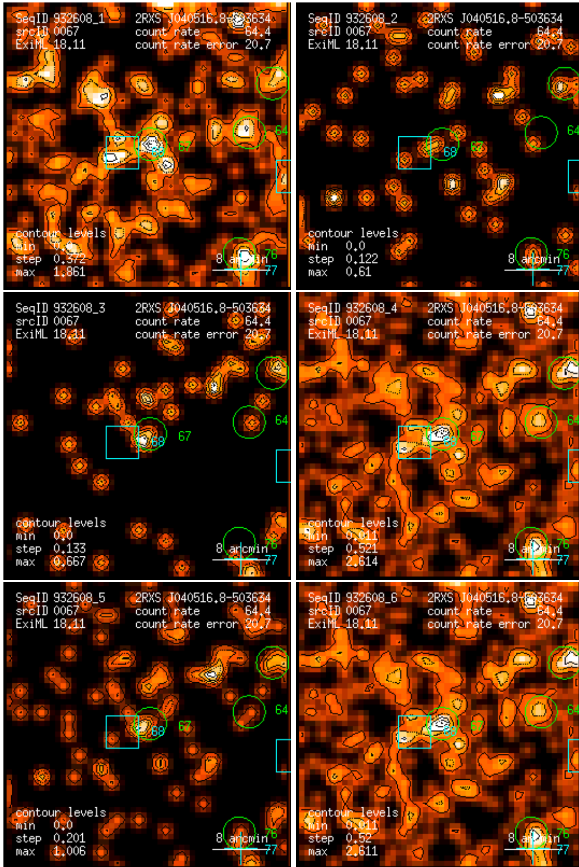
Figure 67: RASS 932608: detection 0067: band rate images, Gaussian filter: (1) PSPC channels 11 – 41, (2) 52 – 90, (3) 91 – 201, (4) 11 – 235, (5) 52 – 201, (6) 11 – 201. Broad band rates in counts/ks. Band rate contour levels in counts/ks/arcmin 2 .
