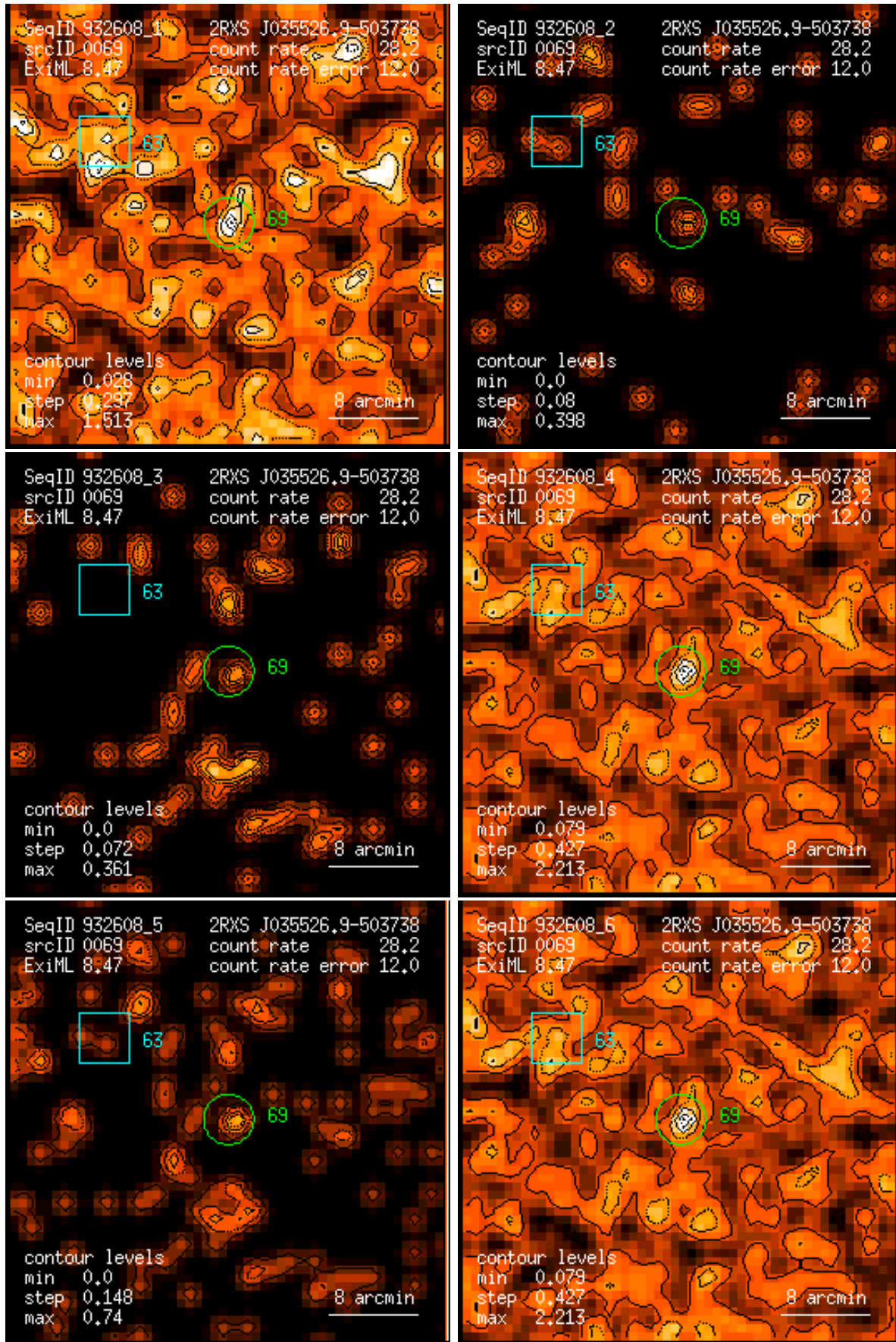
Figure 69: RASS 932608: detection 0069: band rate images, Gaussian filter: (1) PSPC channels 11 – 41, (2) 52 – 90, (3) 91 – 201, (4) 11 – 235, (5) 52 – 201, (6) 11 – 201. Broad band rates in counts/ks. Band rate contour levels in counts/ks/arcmin 2 .
