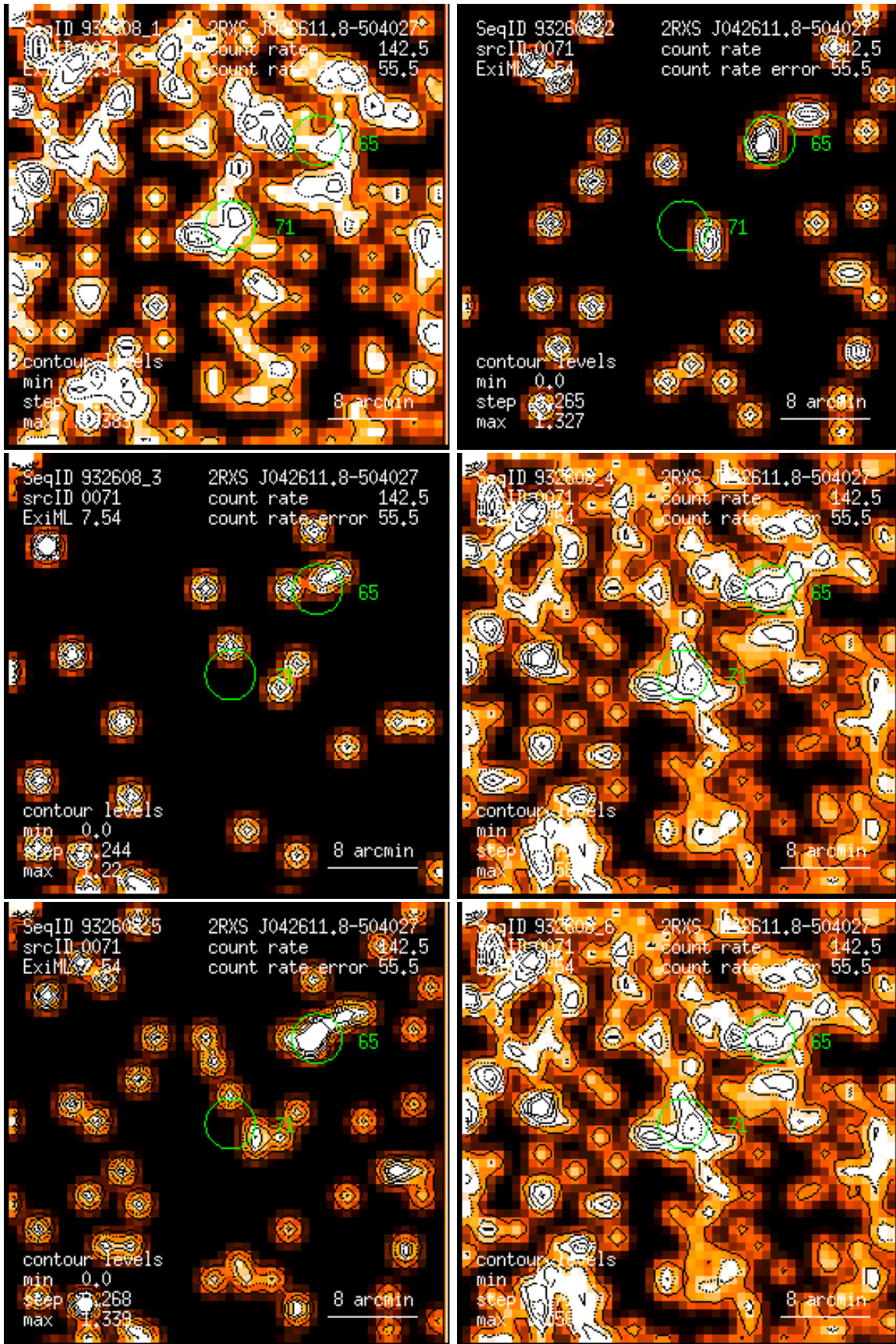
Figure 71: RASS 932608: detection 0071: band rate images, Gaussian filter: (1) PSPC channels 11 – 41, (2) 52 – 90, (3) 91 – 201, (4) 11 – 235, (5) 52 – 201, (6) 11 – 201. Broad band rates in counts/ks. Band rate contour levels in counts/ks/arcmin 2 .
