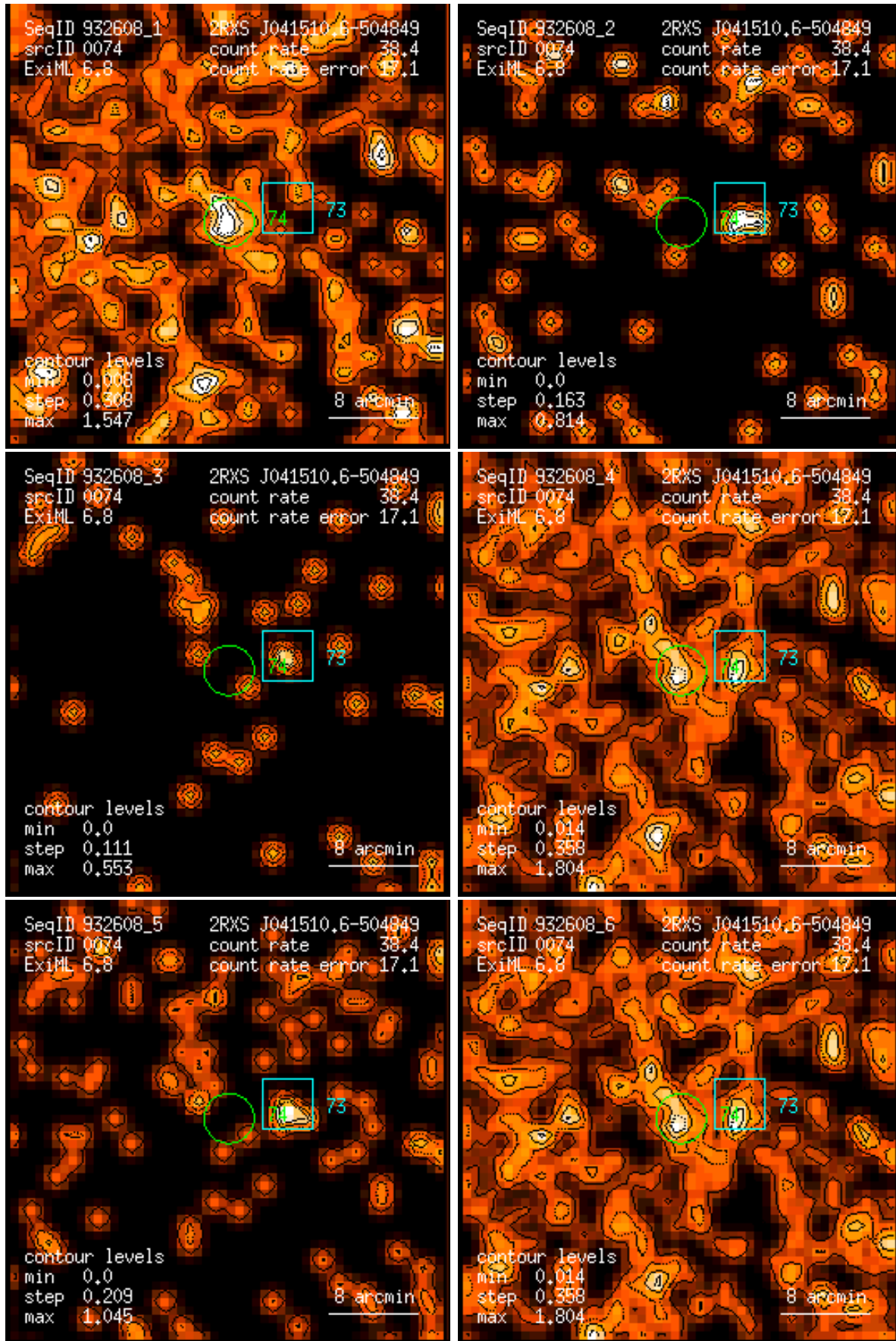
Figure 74: RASS 932608: detection 0074: band rate images, Gaussian filter: (1) PSPC channels 11 – 41, (2) 52 – 90, (3) 91 – 201, (4) 11 – 235, (5) 52 – 201, (6) 11 – 201. Broad band rates in counts/ks. Band rate contour levels in counts/ks/arcmin 2 .
