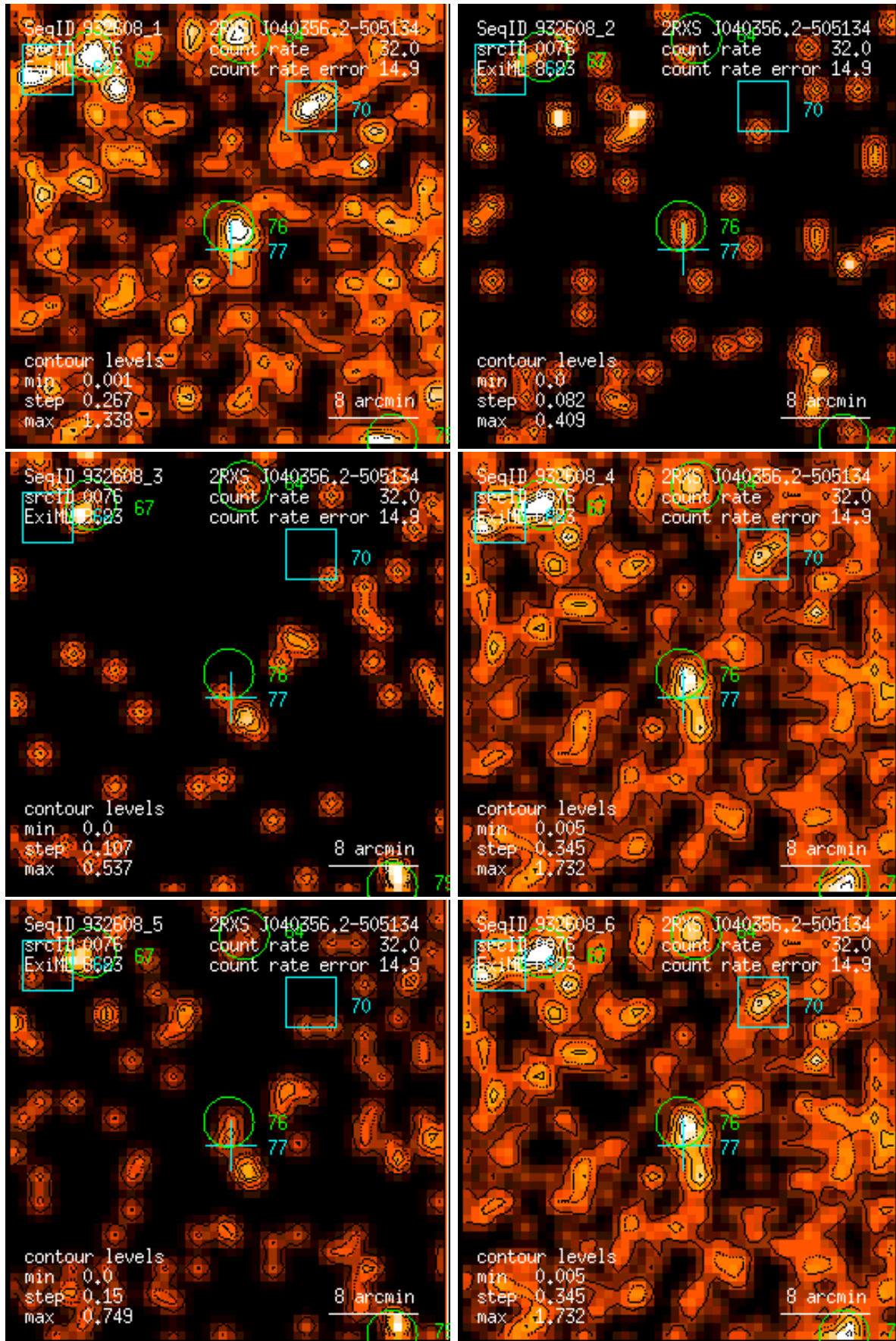
Figure 76: RASS 932608: detection 0076: band rate images, Gaussian filter: (1) PSPC channels 11 – 41, (2) 52 – 90, (3) 91 – 201, (4) 11 – 235, (5) 52 – 201, (6) 11 – 201. Broad band rates in counts/ks. Band rate contour levels in counts/ks/arcmin 2 .
