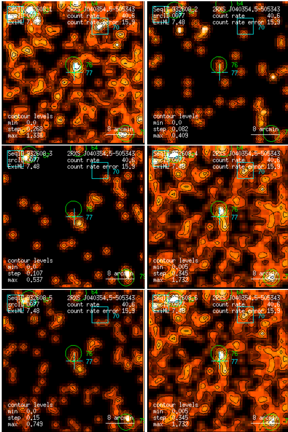
Figure 77: RASS 932608: detection 0077: band rate images, Gaussian filter: (1) PSPC channels 11 – 41, (2) 52 – 90, (3) 91 – 201, (4) 11 – 235, (5) 52 – 201, (6) 11 – 201. Broad band rates in counts/ks. Band rate contour levels in counts/ks/arcmin 2 .
