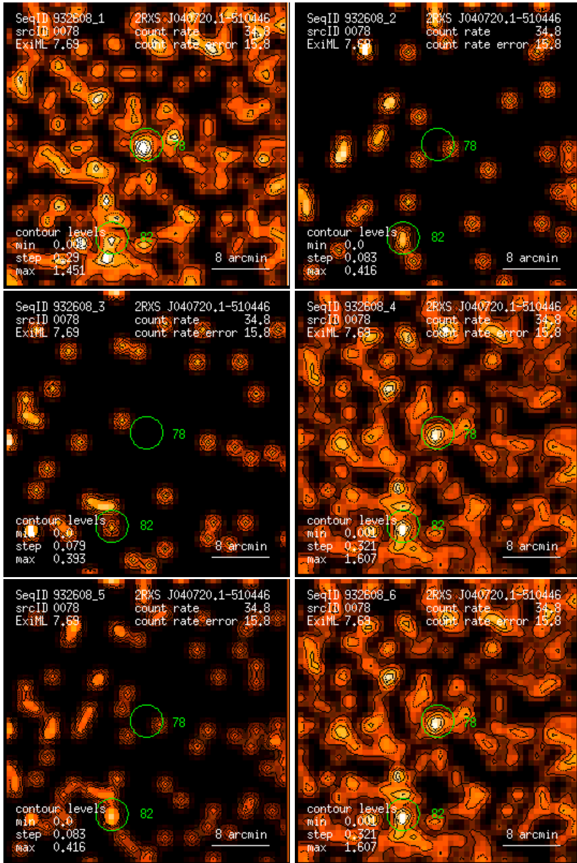
Figure 78: RASS 932608: detection 0078: band rate images, Gaussian filter: (1) PSPC channels 11 – 41, (2) 52 – 90, (3) 91 – 201, (4) 11 – 235, (5) 52 – 201, (6) 11 – 201. Broad band rates in counts/ks. Band rate contour levels in counts/ks/arcmin 2 .
