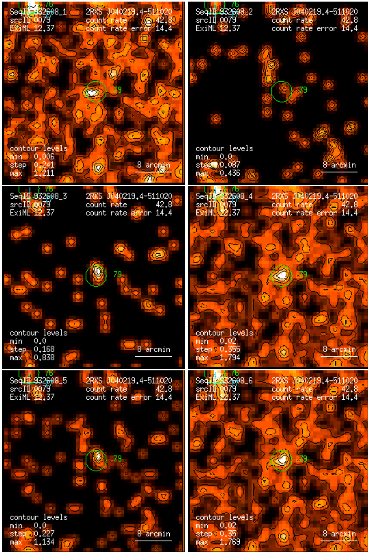
Figure 79: RASS 932608: detection 0079: band rate images, Gaussian filter: (1) PSPC channels 11 – 41, (2) 52 – 90, (3) 91 – 201, (4) 11 – 235, (5) 52 – 201, (6) 11 – 201. Broad band rates in counts/ks. Band rate contour levels in counts/ks/arcmin 2 .
