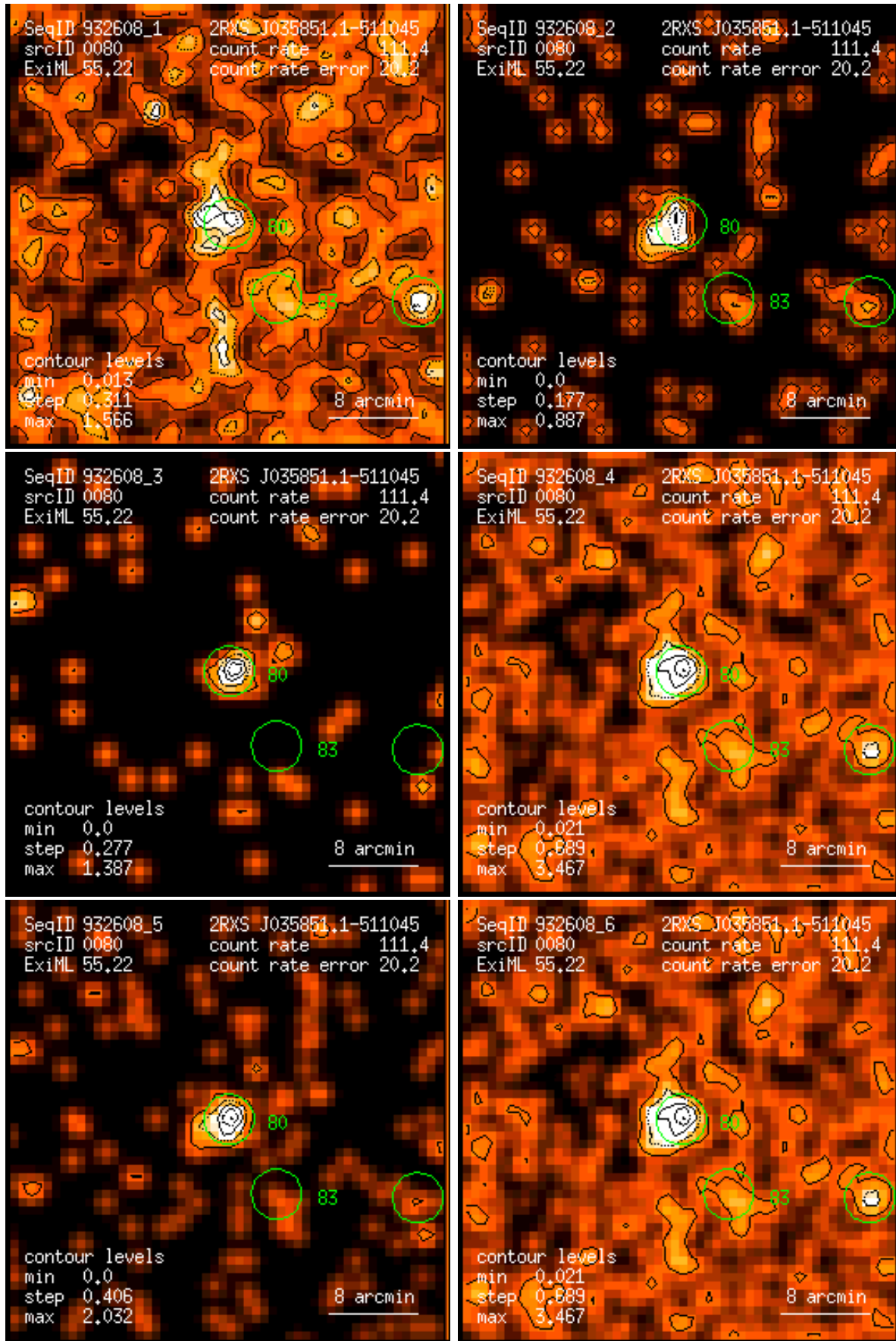
Figure 80: RASS 932608: detection 0080: band rate images, Gaussian filter: (1) PSPC channels 11 – 41, (2) 52 – 90, (3) 91 – 201, (4) 11 – 235, (5) 52 – 201, (6) 11 – 201. Broad band rates in counts/ks. Band rate contour levels in counts/ks/arcmin 2 .
