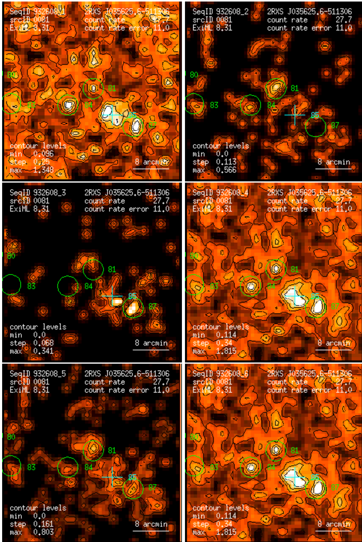
Figure 81: RASS 932608: detection 0081: band rate images, Gaussian filter: (1) PSPC channels 11 – 41, (2) 52 – 90, (3) 91 – 201, (4) 11 – 235, (5) 52 – 201, (6) 11 – 201. Broad band rates in counts/ks. Band rate contour levels in counts/ks/arcmin 2 .
