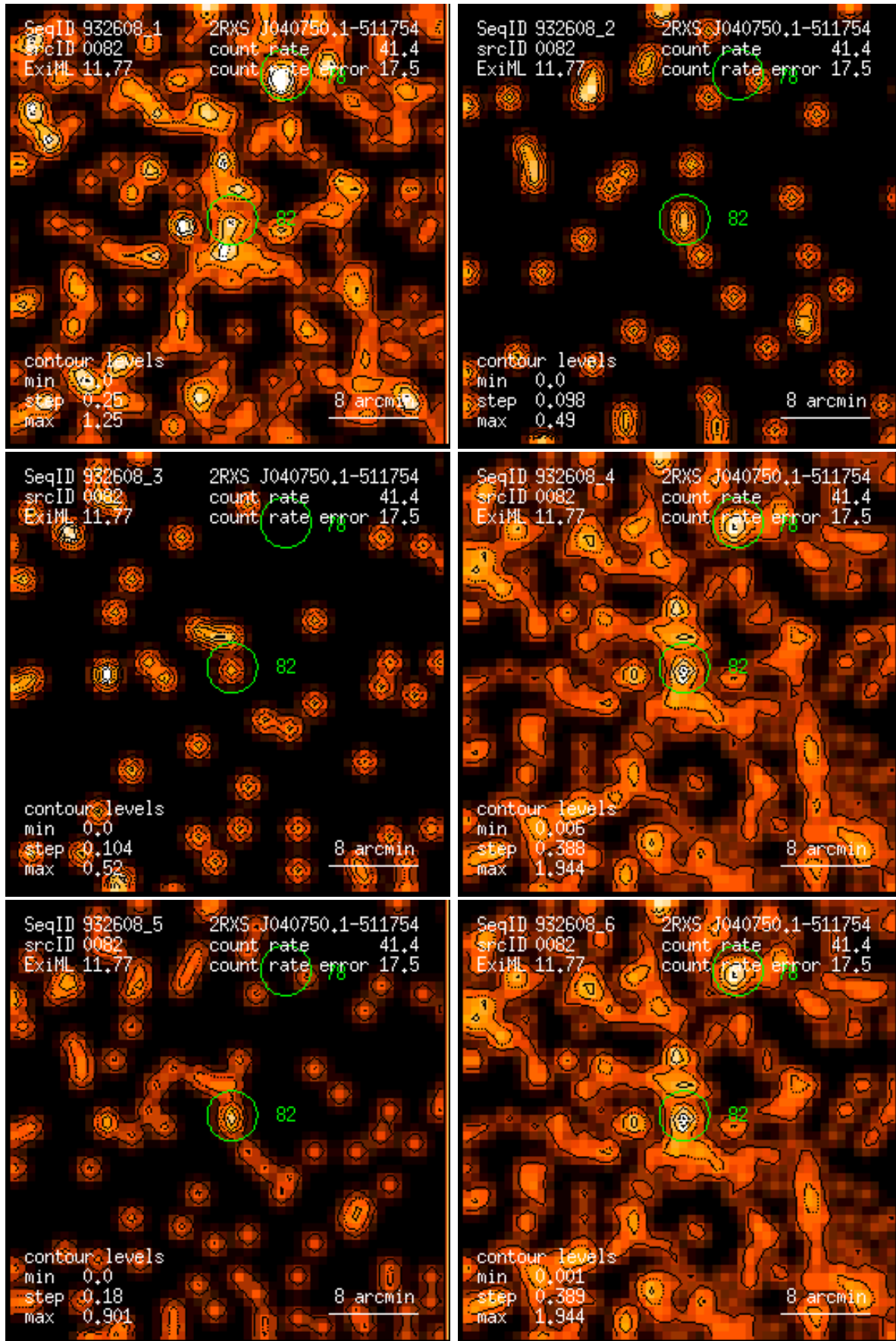
Figure 82: RASS 932608: detection 0082: band rate images, Gaussian filter: (1) PSPC channels 11 – 41, (2) 52 – 90, (3) 91 – 201, (4) 11 – 235, (5) 52 – 201, (6) 11 – 201. Broad band rates in counts/ks. Band rate contour levels in counts/ks/arcmin 2 .
