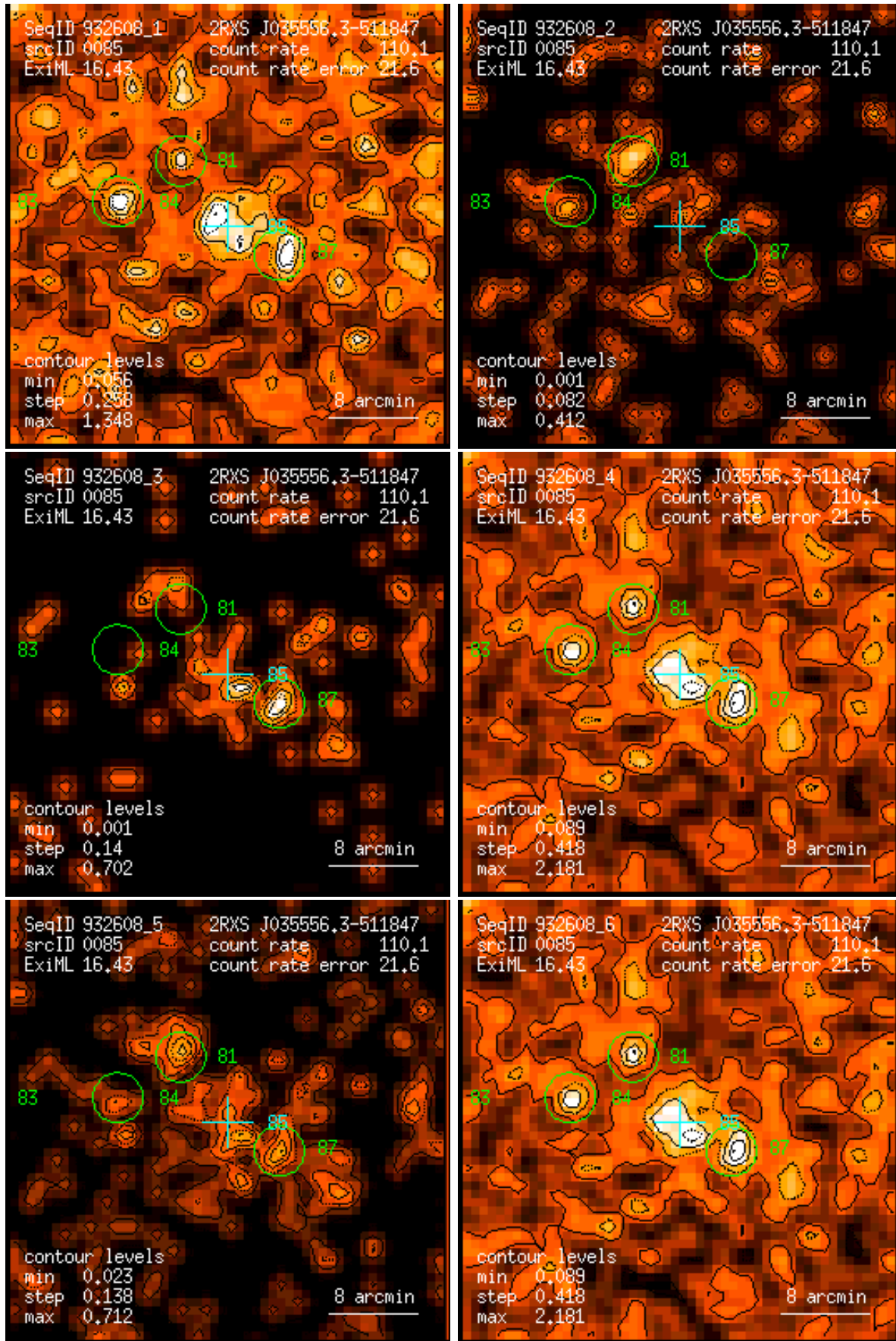
Figure 85: RASS 932608: detection 0085: band rate images, Gaussian filter: (1) PSPC channels 11 – 41, (2) 52 – 90, (3) 91 – 201, (4) 11 – 235, (5) 52 – 201, (6) 11 – 201. Broad band rates in counts/ks. Band rate contour levels in counts/ks/arcmin 2 .
