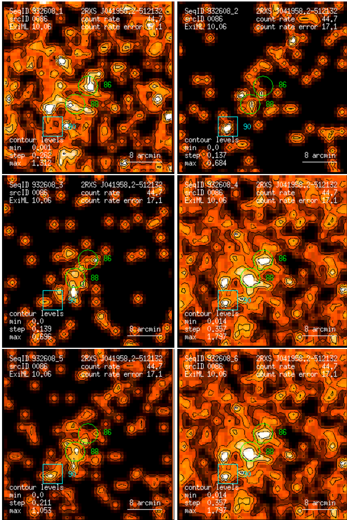
Figure 86: RASS 932608: detection 0086: band rate images, Gaussian filter: (1) PSPC channels 11 – 41, (2) 52 – 90, (3) 91 – 201, (4) 11 – 235, (5) 52 – 201, (6) 11 – 201. Broad band rates in counts/ks. Band rate contour levels in counts/ks/arcmin 2 .
