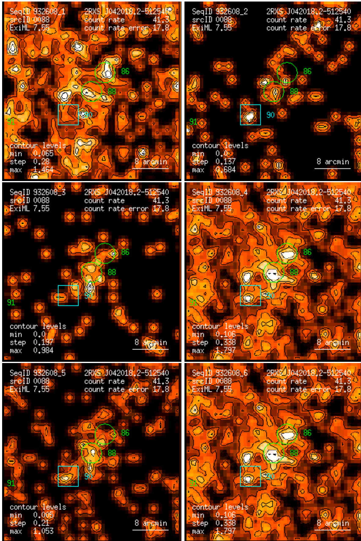
Figure 88: RASS 932608: detection 0088: band rate images, Gaussian filter: (1) PSPC channels 11 – 41, (2) 52 – 90, (3) 91 – 201, (4) 11 – 235, (5) 52 – 201, (6) 11 – 201. Broad band rates in counts/ks. Band rate contour levels in counts/ks/arcmin 2 .
