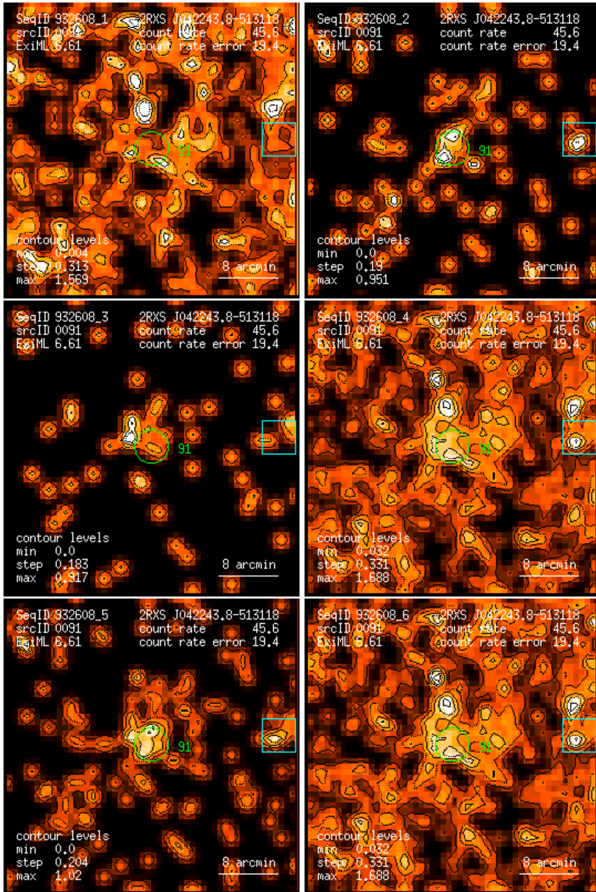
Figure 91: RASS 932608: detection 0091: band rate images, Gaussian filter: (1) PSPC channels 11 – 41, (2) 52 – 90, (3) 91 – 201, (4) 11 – 235, (5) 52 – 201, (6) 11 – 201. Broad band rates in counts/ks. Band rate contour levels in counts/ks/arcmin 2 .
