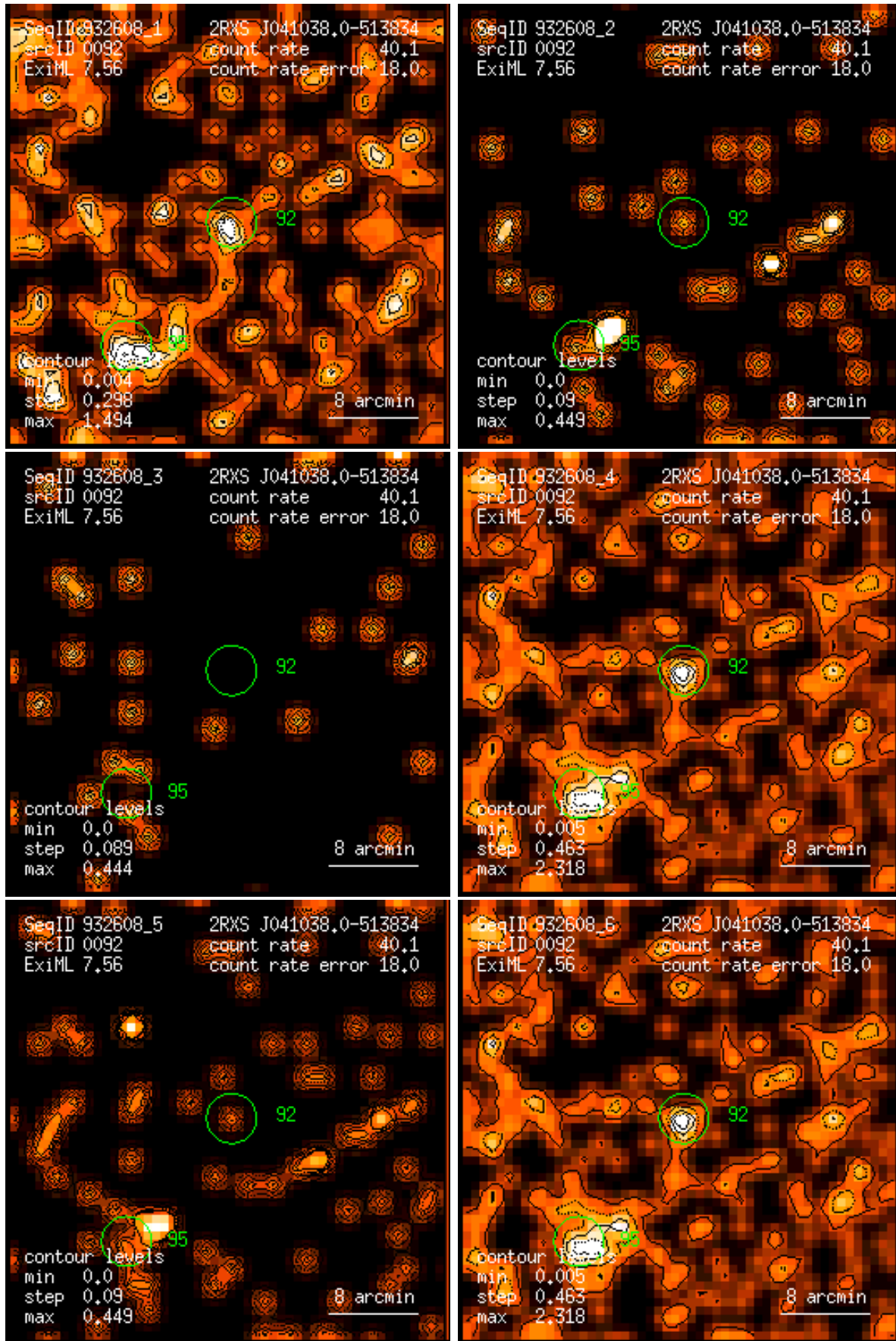
Figure 92: RASS 932608: detection 0092: band rate images, Gaussian filter: (1) PSPC channels 11 – 41, (2) 52 – 90, (3) 91 – 201, (4) 11 – 235, (5) 52 – 201, (6) 11 – 201. Broad band rates in counts/ks. Band rate contour levels in counts/ks/arcmin 2 .
