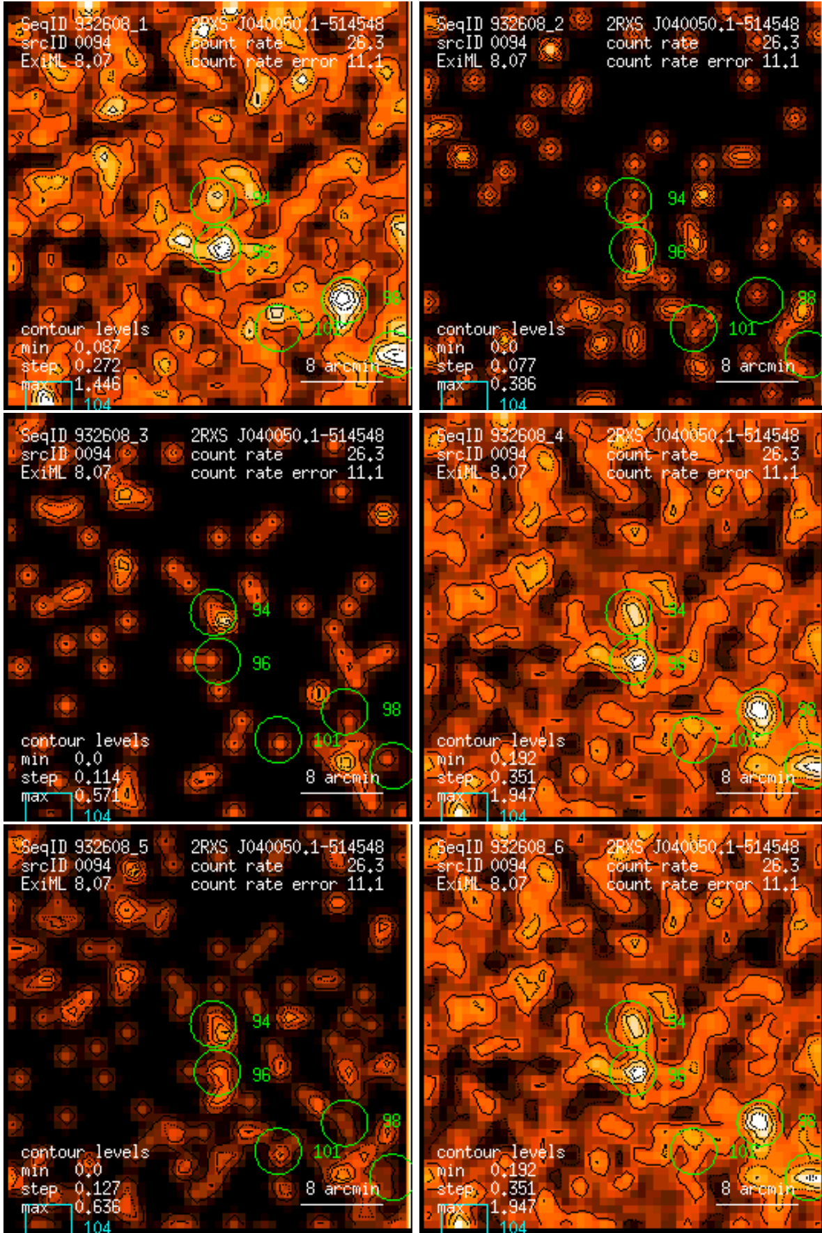
Figure 94: RASS 932608: detection 0094: band rate images, Gaussian filter: (1) PSPC channels 11 – 41, (2) 52 – 90, (3) 91 – 201, (4) 11 – 235, (5) 52 – 201, (6) 11 – 201. Broad band rates in counts/ks. Band rate contour levels in counts/ks/arcmin 2 .
